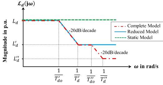
Fig. 2. \mathcal{L}_d(s) magnitude for the three SM models.
