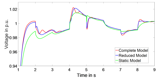
Fig. 8. RMS output voltage for the three SM models.
