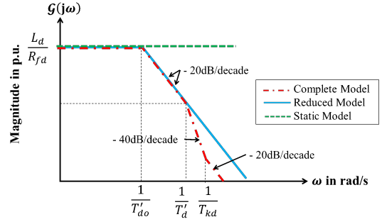
Fig. 3. \mathcal{G}(s) magnitude for the three SM models.
