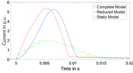
Fig. 9. Output current magnitude defined as |i| = \sqrt{i_d^2 + i_q^2} for the SM models during a three-phases short-circuit of 5 ms.
