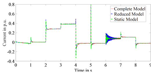
Fig. 5. Output current i_d for the three SM models.
