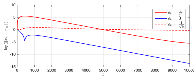
Figure 3: The effect of perturbations, errors in the algorithm (DINAAM-split).
