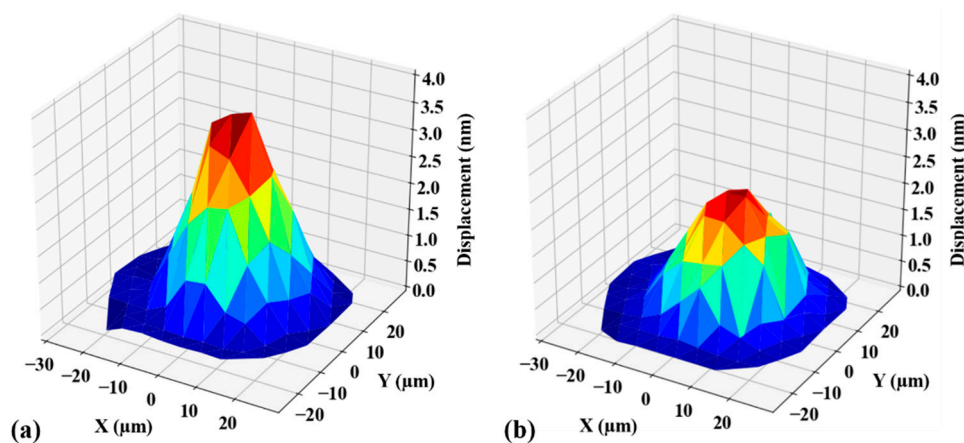
Figure 5. The first resonance mode of the devices working under water load for (a) a control group without PDMS backing (C-PMUT) and (b) B-PMUT.
