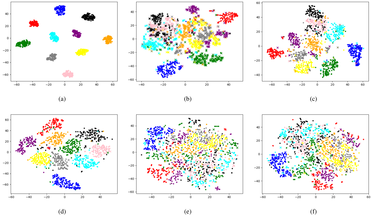
Figure 3. Visualisation of different latent spaces through a 2-dimensional T-SNE [37]. The two axis are the dimensions obtained by the T-SNE. (a) shows the validation (colored digits) latent space, for a model trained normally. (b) shows the test (grey digits) latent space for the same model. (c) shows the validation latent space for a model trained normally, on the original MNIST. (d) shows the validation latent space for a model trained with the RCL-SDG and a margin of 0.9. (e) shows the validation latent space for a model trained with the RCL-SDG without limitation. (f) shows the test latent space for the same model. The color of a dot is its ground truth class (not the same as the colors used for the digits) and its shape represents whether or not the network successfully predicted the correct class: circle if so, cross if not. Best viewed in color.
