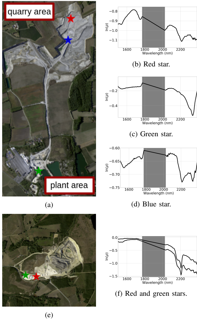
Fig. 11: Hyperspectral images acquired over (a) Cherves-Richemont and (e) Chevenceaux quarries. (b) Gypsum spectrum on the quarry layer. (c) Calcite spectrum from piles used as aggregates. (d) Gypsum-calcite mixture. (f) Kaolinite spectra from two piles.
