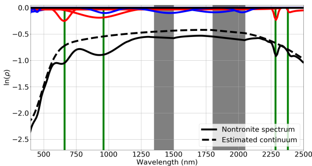
Fig. 8: Nontronite spectrum (black), estimated continuum (black-dashed), diagnostic and secondary EGO Gaussians (red), other Gaussians (blue). The true positions of the diagnostic and secondary absorptions are shown as vertical lines.
