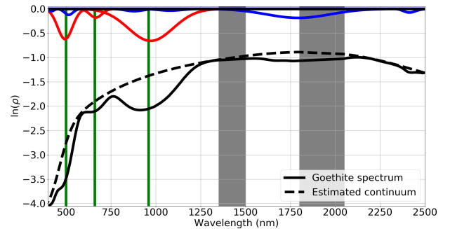
Fig. 6: Goethite spectrum (black), estimated continuum (black-dashed), diagnostic and secondary EGO Gaussians (red), other EGO Gaussians (blue). The true positions of the diagnostic and secondary absorptions are shown as vertical lines.
