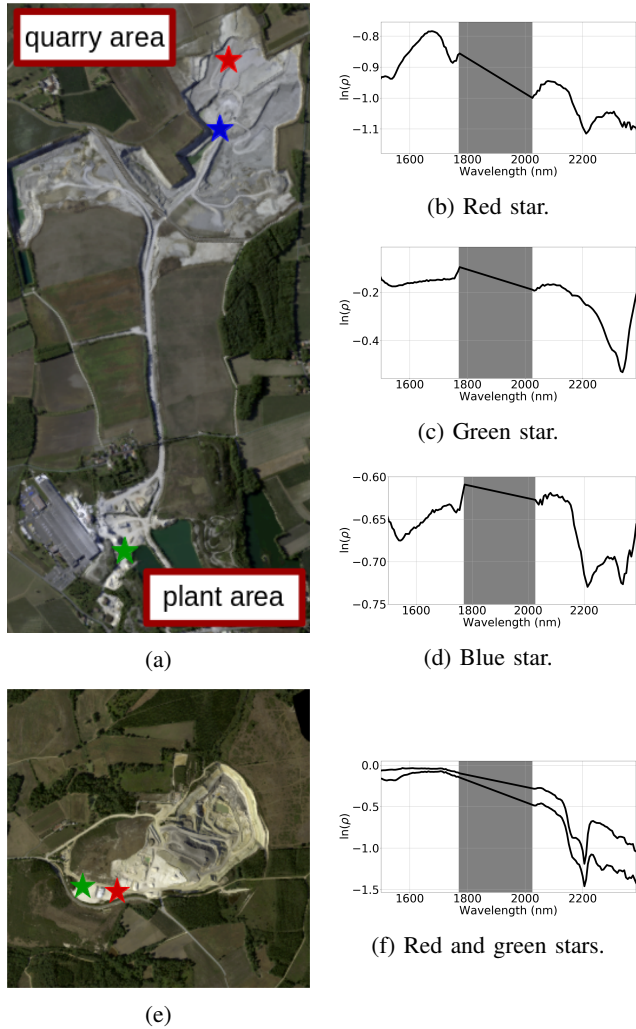
Fig. 11: Hyperspectral images acquired over (a) Cherves-Richemont and (e) Chevaux quarries. (b) Gypsum spectrum on the quarry layer. (c) Calcite spectrum from piles used as aggregates. (d) Gypsum-calcite mixture. (f) Kaolinite spectra from two piles.
