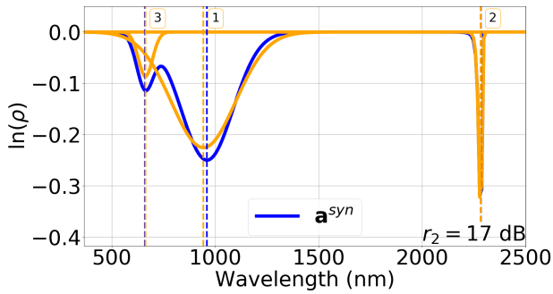
Fig. 5: Synthetic absorption part of spectrum 1 (blue) and EGO Gaussians selected by NNOMP (orange). The order of selection is also indicated. The true absorption positions and their estimates are shown as vertical dashed lines.
