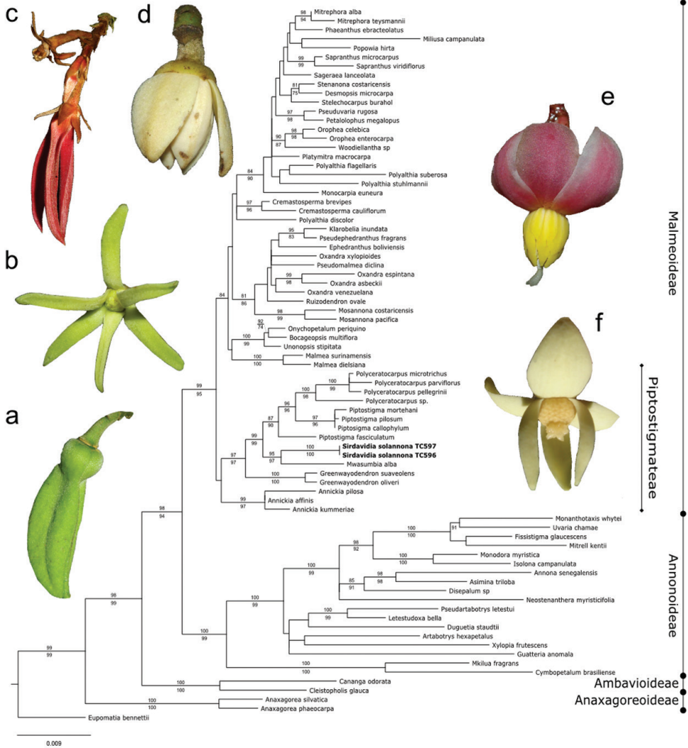
Figure 1. Maximum likelihood tree with support values indicated on branches (ML bootstrap above; MP bootstrap below). Flower morphology of the genera in the Piptostigmataeae tribe. a Annickia affinis (Exell) Versteegh & Sosef b Greenwayodendron suaveolens (Engl. & Diels) Verdc c Piptostigma multinervium Engl. & Diels d Polyceratocarpus parviflorus (Baker) Ghesq e Sirdavidia solannona f Mwasumbia alba . Photos: TLP Couvreur. Note: there is some confusion around the proper identification of the accession Lugas 111 ( Woodiellantha sp in this study).
