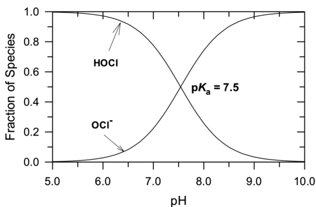
Fig. 2 Speciation of hypochlorite as a function of pH. This figure shows that hypochlorite is mainly present as HOCl below pH 6.0, as about half HOCl half OCl - at pH 7.5, and as OCl - above pH 9.0
