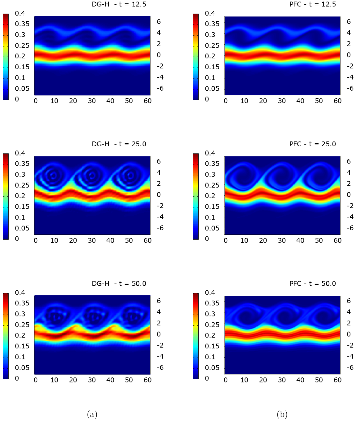
FIGURE 5.6. Bump-on-tail instability: Surface plot of the distribution function f at t = 12.5, 25 and 50 with (a) N_x \times N_H = 64 \times 128 for DG-H and (b) N_x \times N_v = 256 \times 1024 for PFC.
