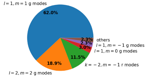
Figure 6. The percentages of different oscillation modes among 960 patterns.
