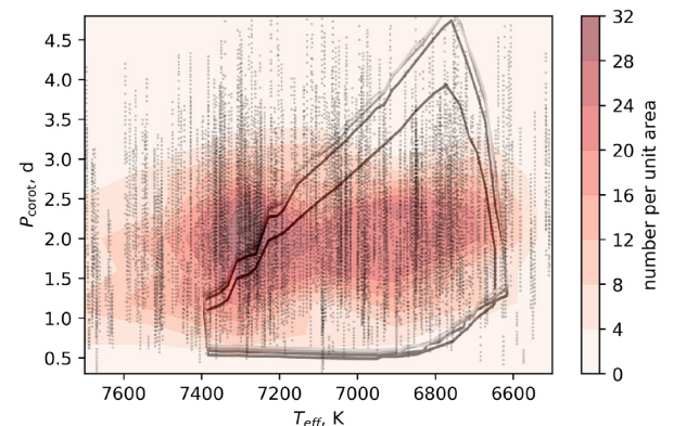
Figure 15. Pulsation period in the corotating frame versus effective temperature. One star has one effective temperature but many pulsation modes, hence the data points (black dots) show vertical fringes. The contour displays the number of the observed pulsation modes. The solid lines show the theoretical areas reported by Bouabid et al. (2013), with equatorial rotation velocities v_{\text{eq}} = 0 (black), 30 (dark grey), 60 (grey), and 90 \text{km s}^{-1} (light grey).
