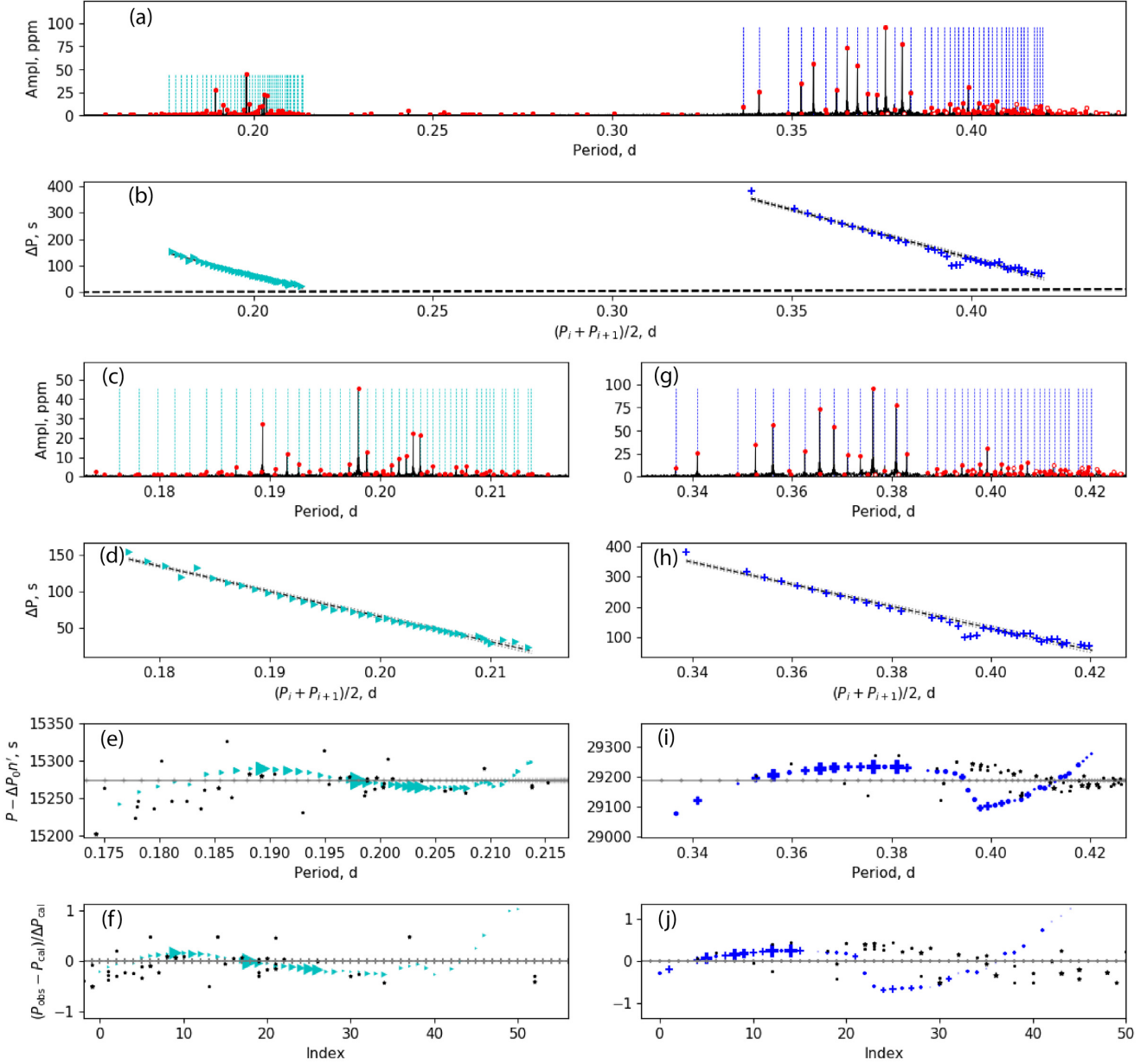
Figure 1. The g-mode patterns of KIC 7694191. Panel (a): the amplitude spectrum with x-axis of period. The y-axis is the amplitude in ppm. The solid red circles present the detected independent frequencies while the open red circles show the combination frequencies. The vertical dashed lines are the linear fits for each pattern. We found two independent frequency groups around 0.20 and 0.38 d. There are two period-spacing patterns. The blue one on the right is the l = 1, m = 1 g modes while the cyan one on the left is the l = 2, m = 2 g modes, whose periods are marked by the vertical dashed lines. Panel (b): the period-spacing patterns of KIC 7694191. The linear fits and uncertainties are shown by the black and grey dashed lines with dips removed. The blue plus symbols are the dipole g modes and the cyan triangle symbols are the quadrupole g modes. Panels (c) and (d): the detail of the spectrum and period-spacing pattern of quadrupole g modes. Panel (e): the sideways Échelle diagram of the quadrupole g-mode pattern. The cyan triangles are the periods belonging to the pattern while the black stars are the noisy peaks. Panel (f): the normalized sideways Échelle diagram of the quadrupole g-mode pattern. Panels (g)–(j): same as (c)–(f) but for the dipole g-mode patterns.
