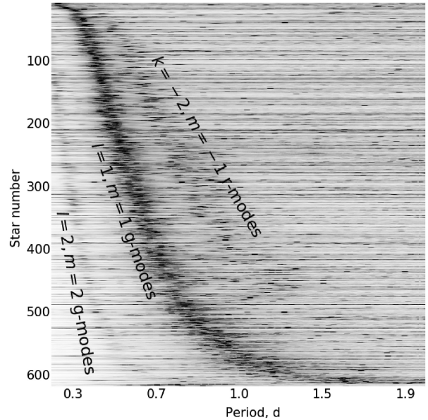
Figure 5. The periodograms of all the \gamma Dor stars with identified period-spacing patterns in our sample. Each row shows the periodogram for one star. The colour stands for the normalized amplitudes to the power of 0.25 for the best visibility. The trends of l = 1, m = 1 g modes, l = 2, m = 2 g modes, and k = -2, m = -1 r modes are seen and marked by the texts.
