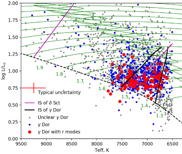
Figure 12. Stars on the HR diagram. The blue points are the \gamma Dor stars with clear g-mode patterns. The red points are the stars with both g- and r-mode patterns. The grey points are the stars we inspected but do not show clear period-spacing patterns. The black lines show the theoretical instability strip (IS) of \gamma Dor star while the purple lines depict the observed IS of \delta Sct star by Murphy et al. (2019).
