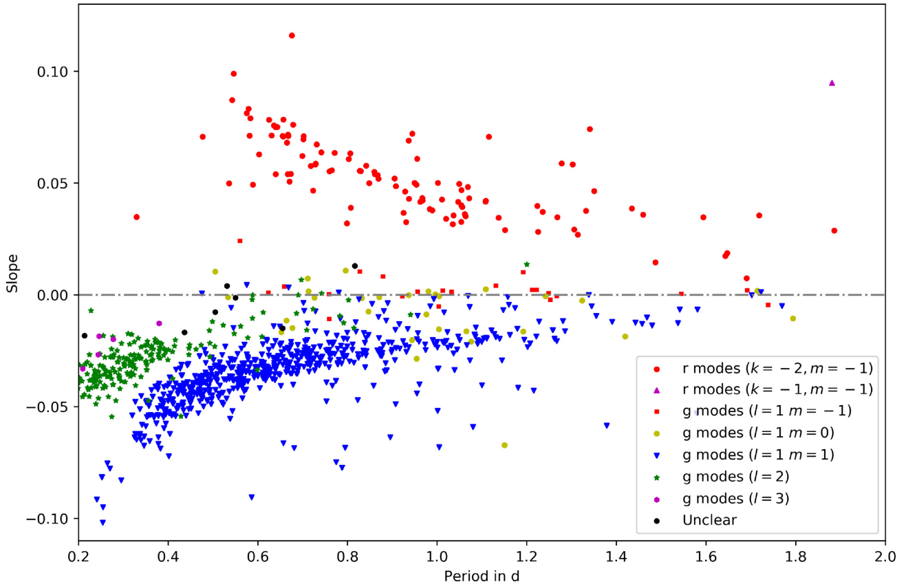
Figure 8. Slopes versus the means of the periods of 960 period-spacing patterns from 611 \gamma Dor stars. The x -axis is the mean period in each pattern. The y -axis is the slope between the period spacing and the period with dips removed. Different colours and symbols show different modes.
