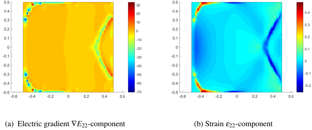
FIG. 6: (a) Electric field gradient component \nabla E_{22} and (b) strain component \epsilon_{22} within the PZT-PVDF microstructure corresponding to the optimized coefficient \bar{K}_{2222} .
