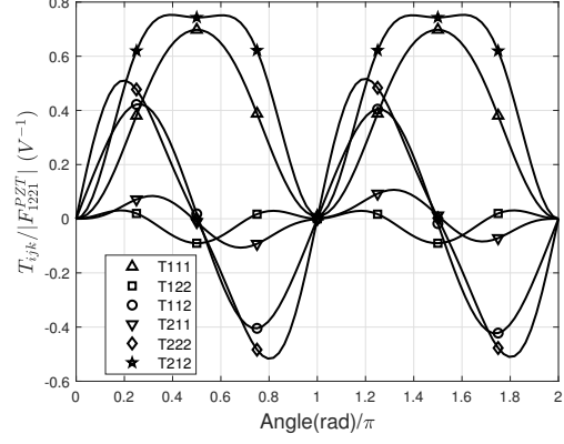
(b) Evolution of \bar{T} tensor components
