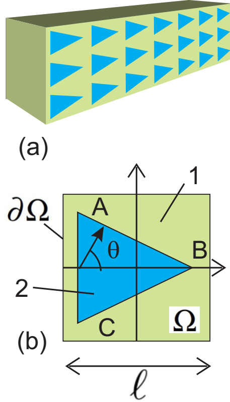
FIG. 1: (a) Periodic piezoelectric structure; (b) Representative Volume Element (RVE). Both matrix phases (phase 1) and inclusion (phase 2) are made of the same piezoelectric material, but rotated by a mismatch angle \theta .
