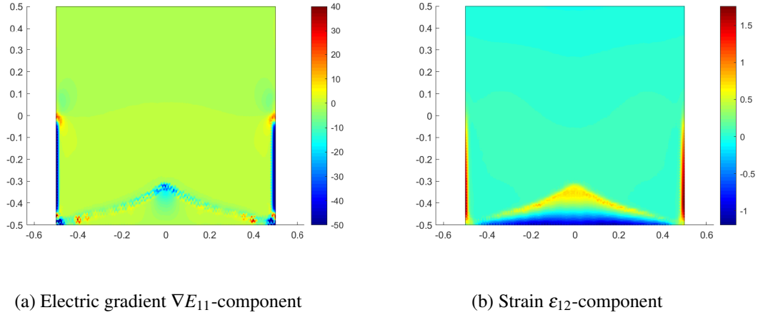
FIG. 7: (a) Electric field gradient component \nabla E_{11} and (b) strain component \epsilon_{12} within the PZT-PVDF microstructure corresponding to the optimized coefficient \bar{K}_{1211} .
