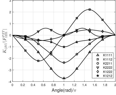
(a) Evolution of \bar{K} tensor components
