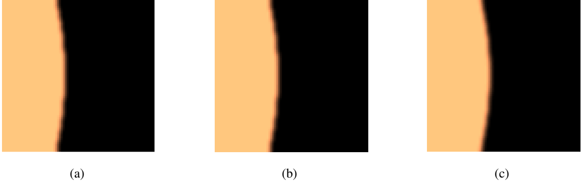
FIG. 3: Optimal topology for \bar{K} for the PZT/PZT composite: (a) \bar{K}_{1111} ; (b) \bar{K}_{2211} ; (c) \bar{K}_{1212} .
