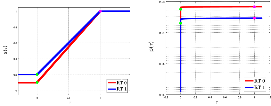
Figure 13: Parametrized saturation and pressure functions using the Brooks and Corey model and parameters of Table 1. The green dot indicates the value for \tau = \tau_* and the magenta one \tau = \tau_s .
