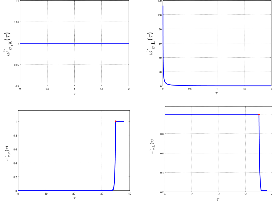
Figure 17: Comparison between \omega'_{\sigma,K}(\cdot), \omega'_{\sigma,L}(\cdot) (above) and \omega'^2_{\sigma,K}(\cdot), \omega'^2_{\sigma,L}(\cdot) (below) when using steep capillary pressure curves.
