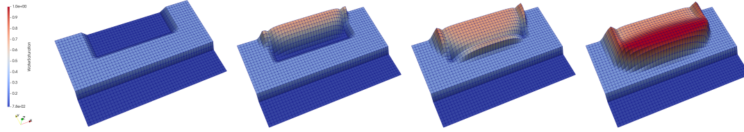
Figure 20: Evolution of the saturation profile for t \in \{0s, 21.5 \cdot 10^3s, 41.5 \cdot 10^3s, 86.4 \cdot 10^3s\} for the non-steep filling case using Van Genuchten model, Method B and the 50 \times 30 cells mesh.
