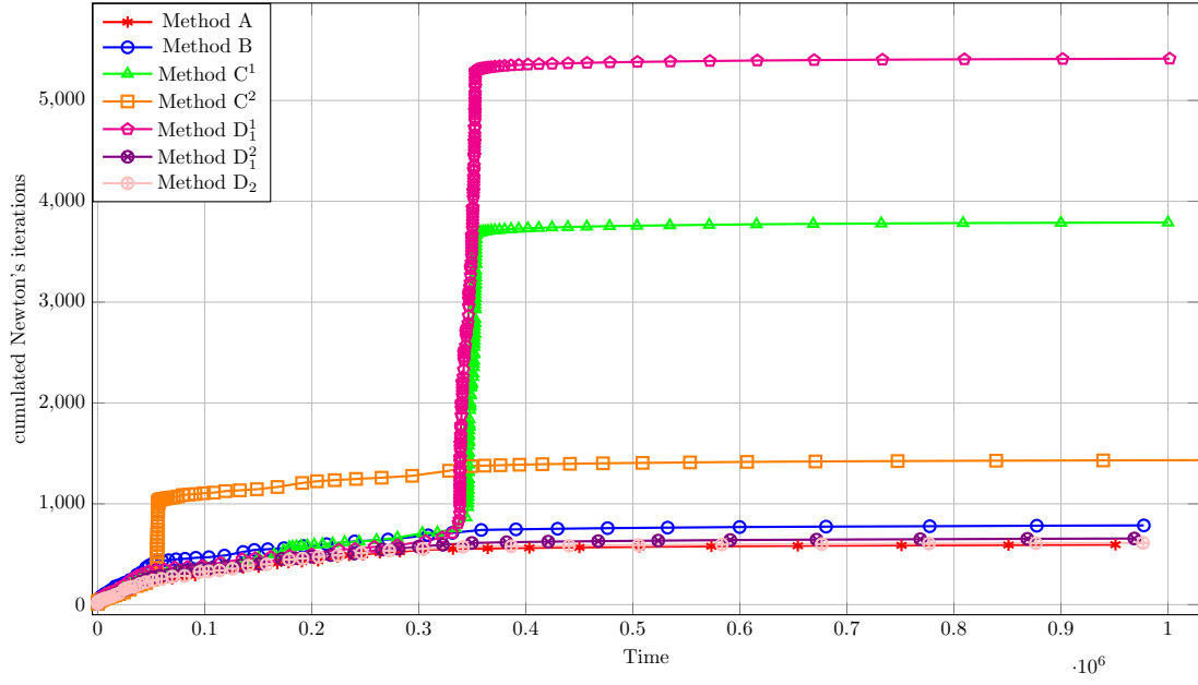
Figure 26: Steep drainage case: Evolution of the cumulated number of Newton's iterations for the 50 \times 30 cells mesh
