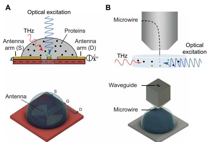
Fig. 8. THz spectroscopy experimental setups. (A) Rectenna for the 0.07 to 0.11 THz band. (B) Microwire-based probe for the 0.25- to 0.37-THz band.
