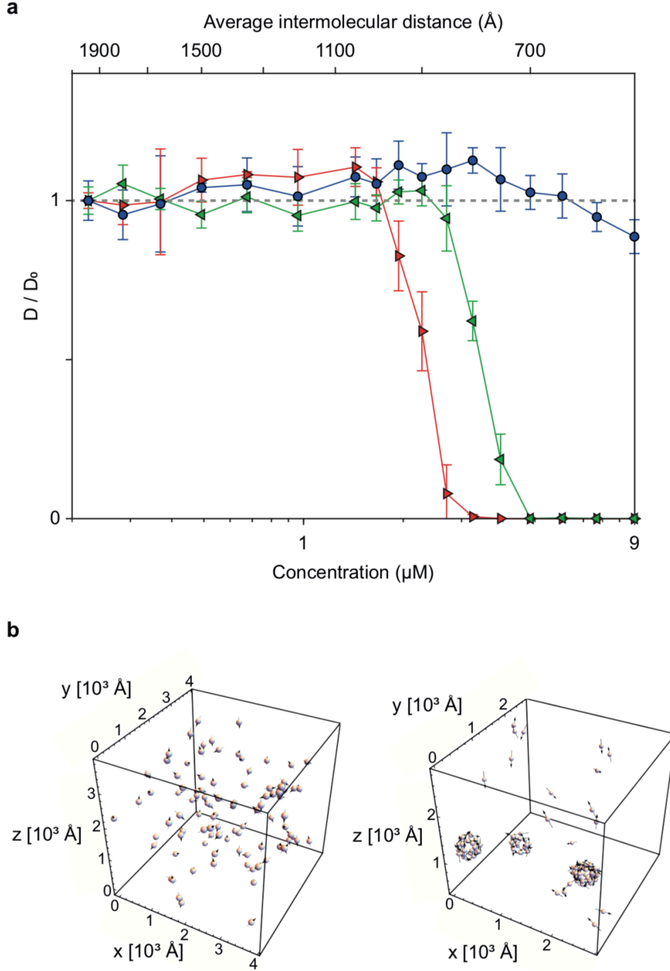
Figure 3: Effect of protein concentration and laser power illumination on R-PE diffusion: Clustering phase transition. (a) Diffusion coefficients normalized to the Brownian D_0 values measured for each data series at 0.223 \mu\text{M} ( \langle r \rangle \simeq 1950 \text{ \AA} ) and recorded at 50 \mu\text{W} (blue circles), 100 \mu\text{W} (green triangles), and 150 \mu\text{W} (red triangles). Each point corresponds to the average of 5 independent experiments. (b) Snapshots of numerical Monte Carlo computations involving long-range electrodynamic inter-particle forces obtained with different initial values of \langle r \rangle . With \langle r \rangle_{\text{initial}} \simeq 1000 \text{ \AA} the system remains in the dispersed phase (lower left box) where D/D_0 = 1 (Brownian diffusion); with \langle r \rangle_{\text{initial}} \simeq 950 \text{ \AA} the system switches to the clustered phase with D/D_0 very small (lower right box).
