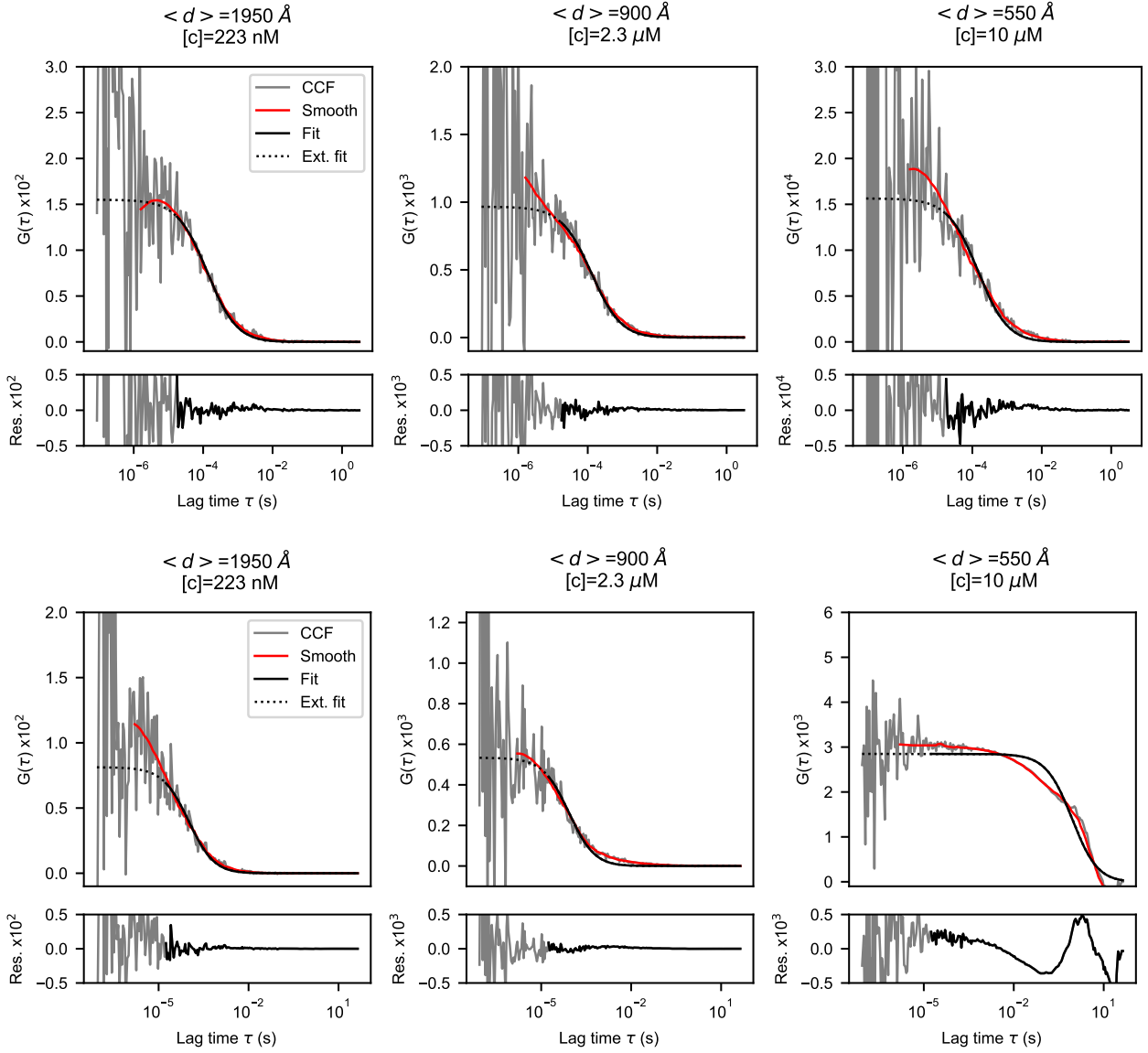
Figure 12: Cross-Correlation Functions (CCFs) for R-PE solutions at different concentrations. From left to right the average intermolecular distances are: \langle d \rangle = 1950 \text{ \AA} , \langle d \rangle = 900 \text{ \AA} , \langle d \rangle = 550 \text{ \AA} , respectively. The upper panels display the results obtained with a laser power input of 50 \text{ μW} (grey lines). The lower panels display the results obtained with a laser power input of 150 \text{ μW} (grey lines). A Savitzky-Golay filter is used to smooth the CCFs (red lines), and to consequently obtain the diffusion time \tau_D at Half Height (THH). Fits of the CCF are also shown (black lines), and the extended fits (outside of the original fitting range) are represented with dashed lines. Residuals of the fits are also plotted: the black lines correspond to the standard residuals, and the grey lines to the extended residuals. At the highest concentration, for \langle d \rangle = 550 \text{ \AA} , and laser power input of 150 \text{ μW} , the correlation time is increased by several orders of magnitude, entailing a drop of the diffusion coefficient by the same amount.
