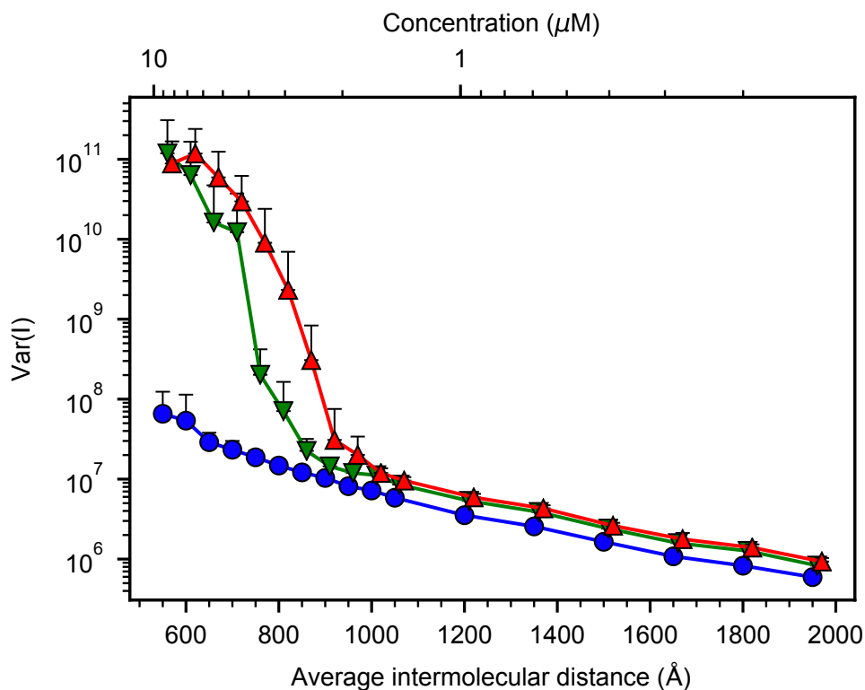
Figure 11: Variance of the fluorescence intensity recorded for R-PE solutions at different laser power input: 50 \mu W (blue circles), 100 \mu W (green down-pointing triangles), and 150 \mu W (red up-pointing triangles). Only upper error bars are shown on this plot for convenience, as the y axis is on a logarithmic scale.
