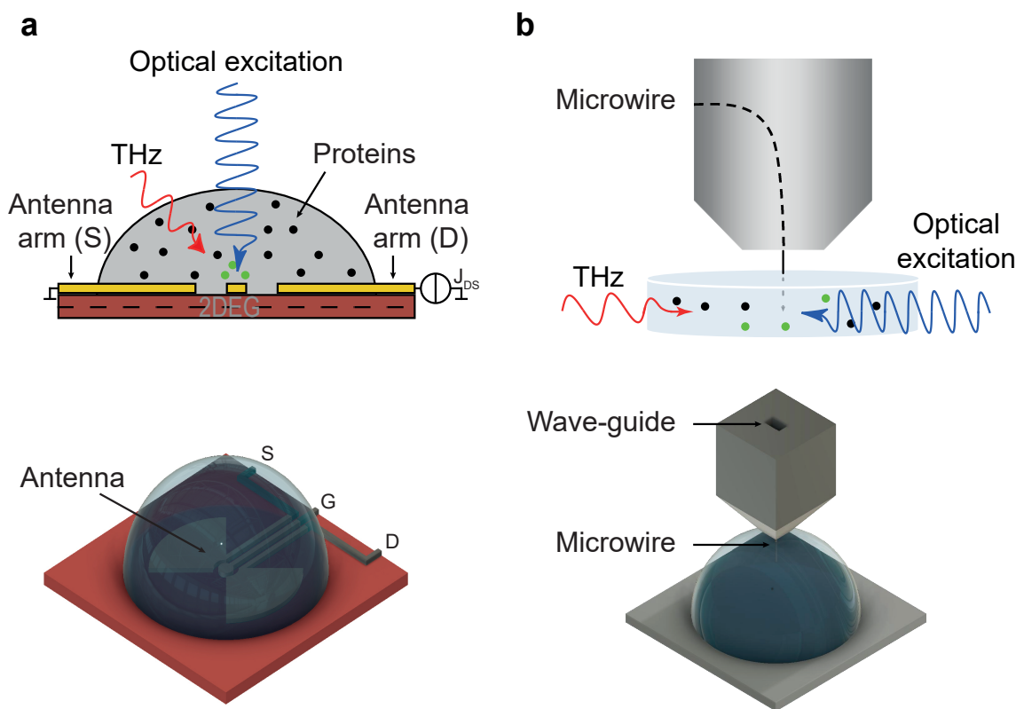
Figure 5: THz-spectroscopy experimental setups. (a) Rectenna for the 0.07 to 0.11 THz band; (b) Microwire-based probe for the 0.25 to 0.37 THz band.
