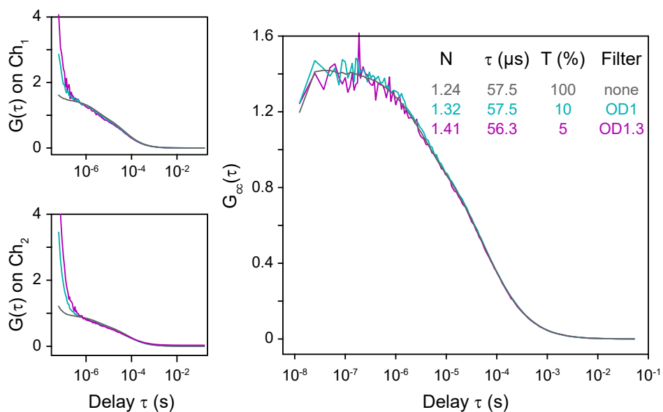
Figure 7: CCFs in the presence of micro-molar concentrations of fluorescent dyes obtained with density filters along the optical path combined with averaging during long acquisition times. The left panel shows the comparison of Cross-Correlation Functions (CCFs) of a single solution of the dye Atto 488 at the concentration of 1 nM, measured without OD (Optical Density) filter (no OD, black line) along the fluorescence path, with OD1 and with OD1.3 (cyan and magenta lines, respectively). Panels on the right show the Auto-Correlation Functions (ACFs) obtained with the signals of channels 1 and 2 for the same measurements. At short time-lag the ACFs clearly show a sharp increase, whereas this phenomenon is absent on CCFs. The phenomenon is consequently an artifact attributed to afterpulsing. Each CCF was obtained by averaging 72 CCFs, each one obtained from a record of 50 seconds, corresponding to an overall acquisition time of one hour.
