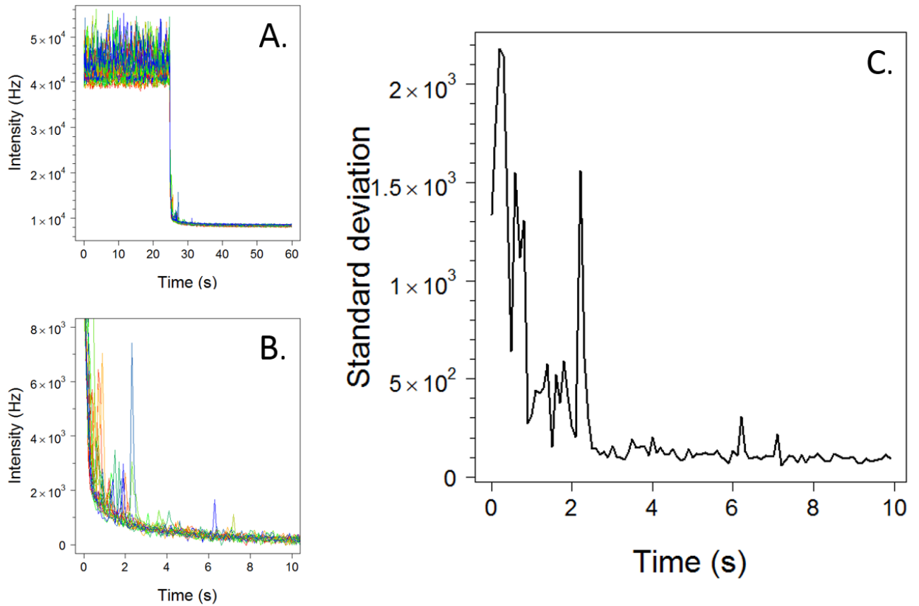
Figure 13: Decay of the clusters of R-PE induced by a sudden lowering of the laser power density. The results reported here have been obtained using ten samples corresponding to an average intermolecular distance of 650 \text{ \AA} . On panel A, the laser input has been lowered from 150 \text{ \mu W} to 50 \text{ \mu W} at t = 25 \text{ s} . Panel B is a zoom of panel A, starting at t = 25 \text{ s} . Panel C is the standard deviation of the intensity of the different samples recorded and displayed by panels A and B. Here the thermal fluctuations overcome the attractive electrodynamic forces weakened by the lowering of the energy input rate, thus destroying the clusters. The initial time t = 0 has been arbitrarily chosen in the already clustered phase.
