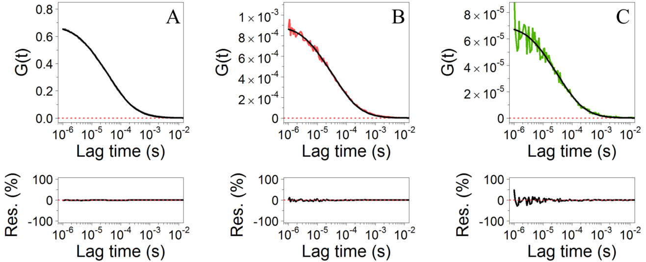
Figure 8: FCCS results at high concentrations of fluorescent molecules and using density filters. Panels A to C display the CCFs - as shown in Figure 7 - corresponding to solutions of 1 nM, 1 \mu M, and 10 \mu M of Atto 488 dye using no OD filter, OD1, and OD1.3 filters, respectively. Each CCF was obtained by averaging 72 CCFs, each one obtained from a record of 50 seconds, corresponding to an overall acquisition time of one hour. The fitting curves are also displayed in black on each panel, and the residuals are visible below each CCF (displayed in percentage). The same values of \tau reported in Figure 7 are found within a 2% deviation.
