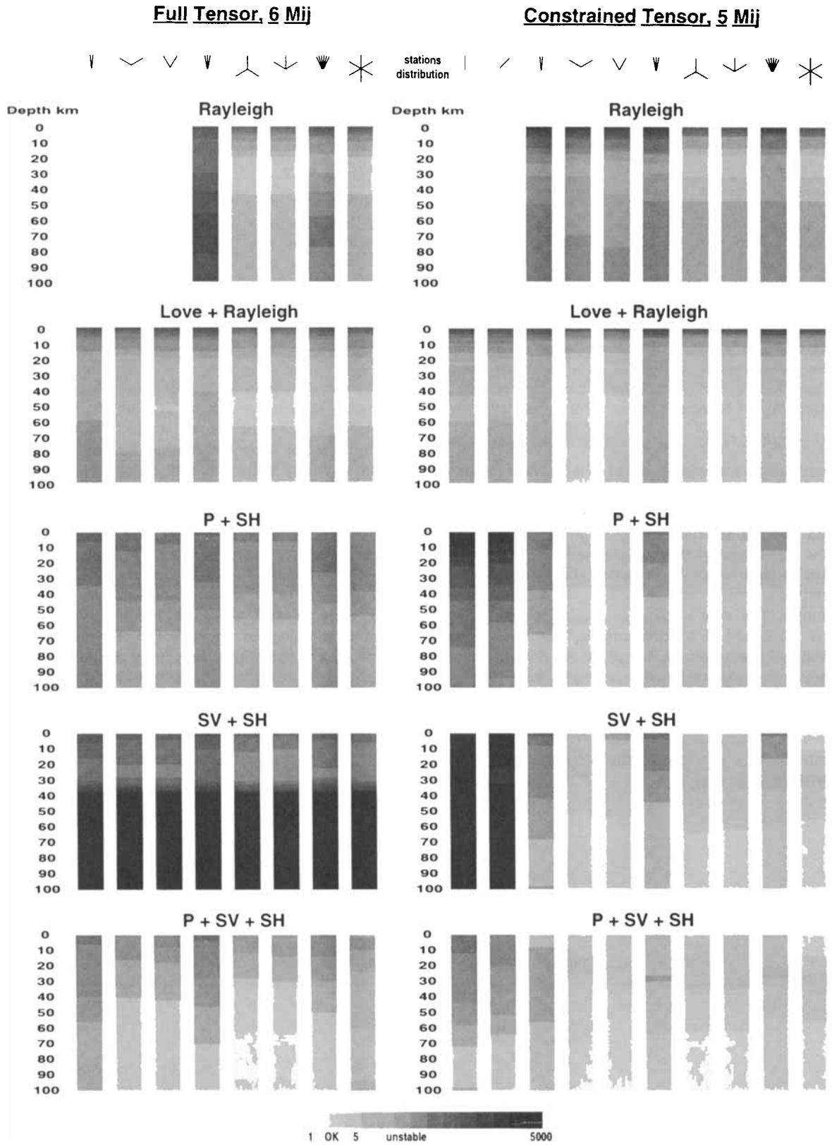
Figure 2. Tables of condition numbers of teleseismic moment tensor inversions, using different combinations of stations and components. The station distribution is symbolized on the top, and the grey scale codes the condition number as indicated at the bottom. The left part concerns full moment tensor inversions, the right part deviatoric ones. The values of the condition number are indicated for depths of 0–100 km. The period range is 10–60 s for body waves and 30–300 s for surface waves.
