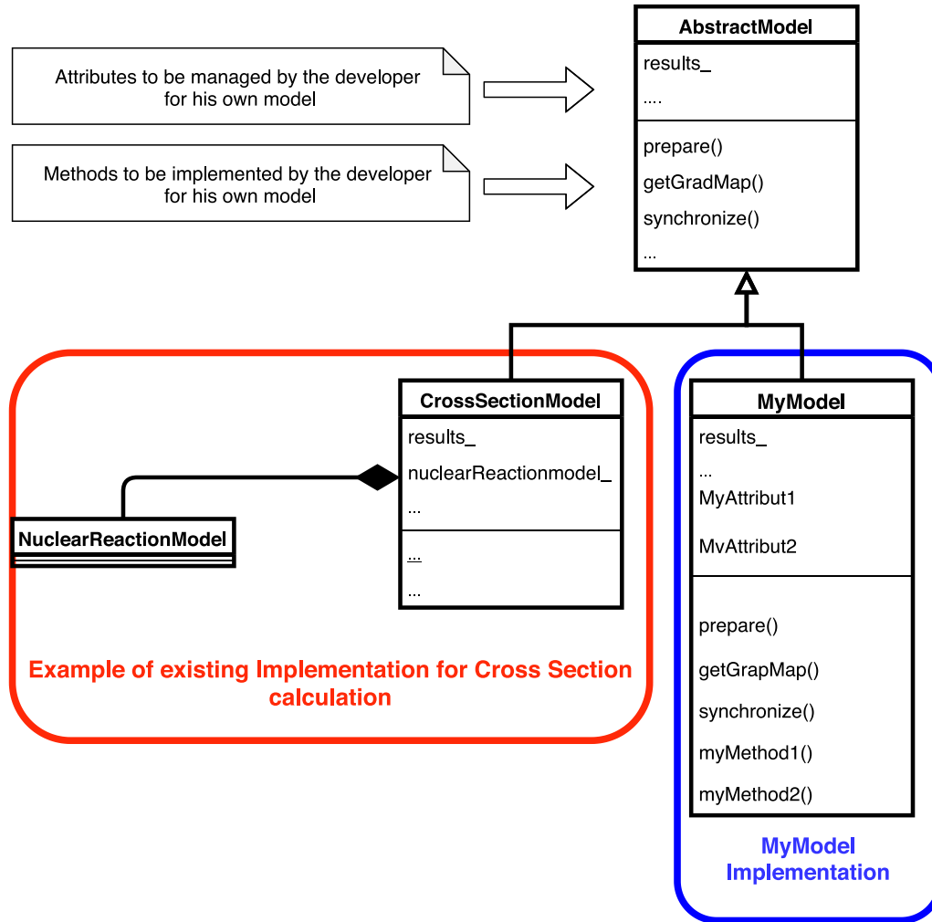
Fig. 1. UML diagram description of CONRAD AbstractModel interface. The API for model implementation (called specialization) is presented.
