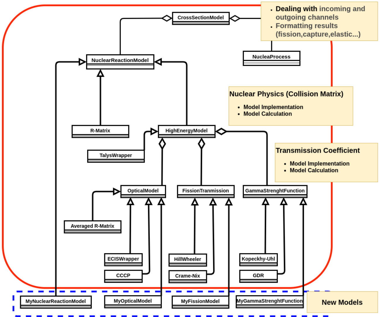
Fig. 3. Simple diagram description of CONRAD CrossSectionmodel interface. The API for new models implementation (called specialization) for cross section is presented. The red box contains existing implementations and the blue one deals with new models development and the appropriate interface with existing code.
