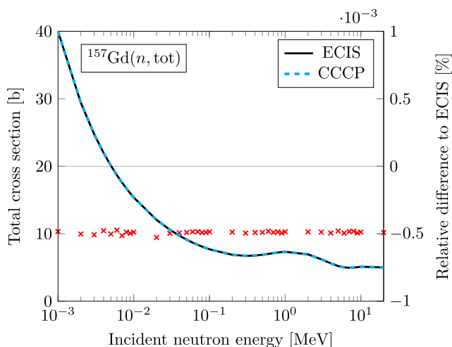
Fig. 6. ECIS06/CONRAD (aka CCCP) total cross section comparisons on ^{157}\text{Gd} .
