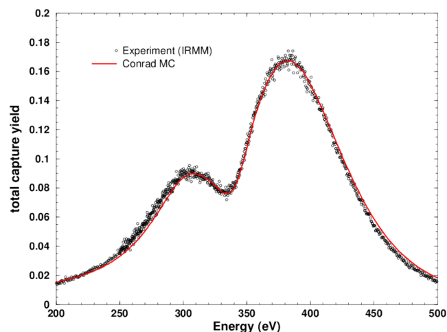
Fig. 5. Comparison between experimental values and theoretical description with multiple-scattering corrections for ^{55}\text{Mn} neutron induced capture yields. Figure taken from [13].
