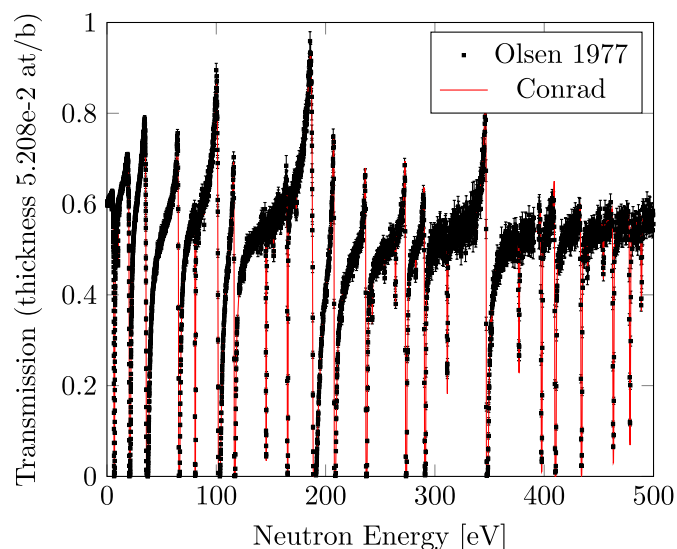
Fig. 4. Comparison between experimental values and theoretical description for ^{238}\text{U} neutron induced transmission. Figure taken from [11].
