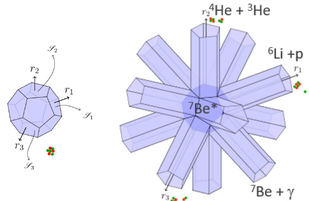
Fig. 12. Schematic view of the ^7\text{Be} compound nucleus with channel surfaces and radii (left) and formation and decay through various channels (right).
