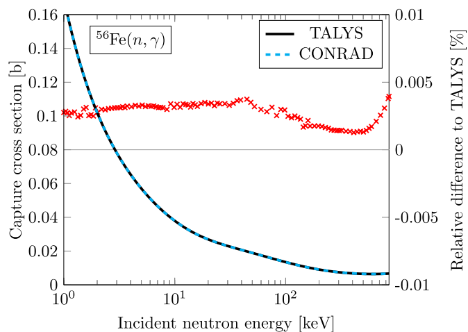
Fig. 7. TALYS1.4/CONRAD ( n,\gamma ) cross section comparisons on ^{56}\text{Fe} .
