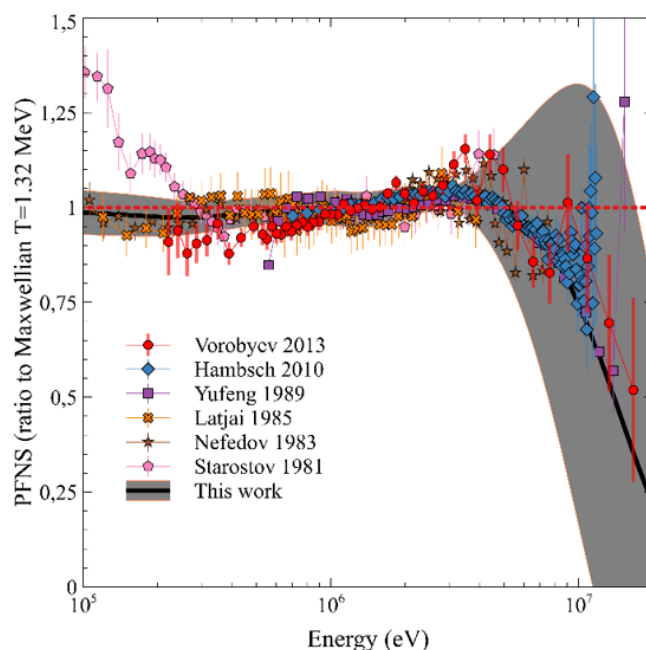
Fig. 9. ^{235}\text{U} thermal neutron induced prompt fission neutron spectra evaluation with CONRAD. Comparison between experiment and theory (Madland-Nix Los Alamos model) are given, as well as an uncertainty evaluation. Figure courtesy of A. Chebboubi.
