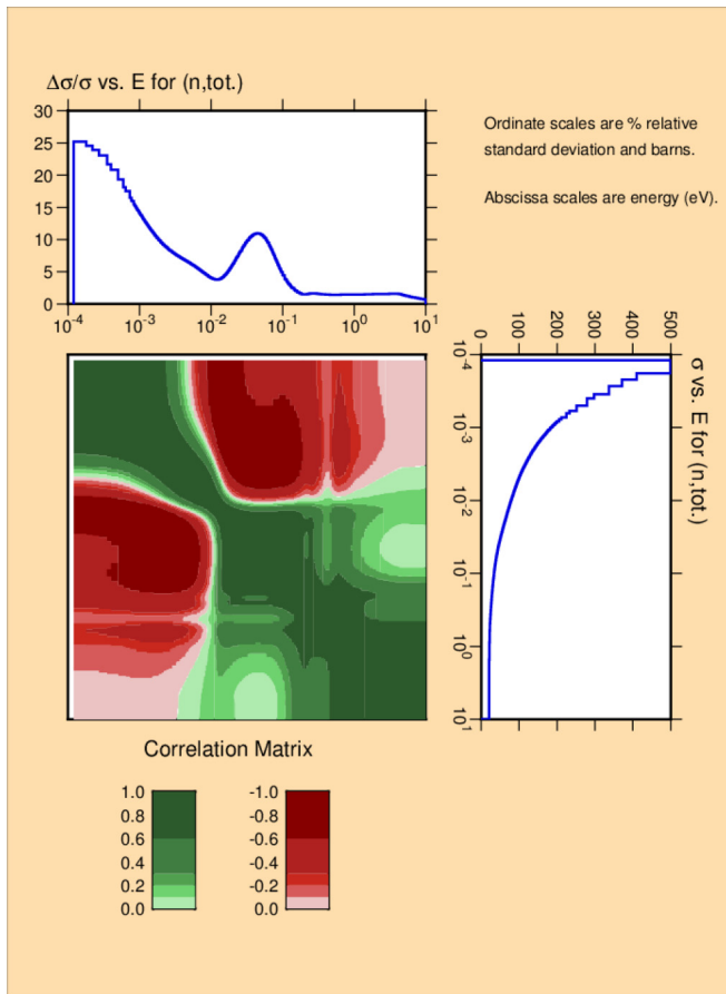
Fig. 10. Relative uncertainties and correlation matrix for the total cross section of H in H 2 O at 574K obtained with the Miscellaneous analysis mode of CONRAD by using the TSL parameters of JEFF-3.1.1.
