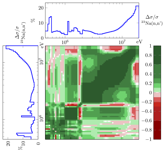
Fig. 8. New covariance evaluation with CONRAD of ^{23}\text{Na} ( n, n' ) cross section [35] based on the analysis of JRC/Geel inelastic cross section measurements [36]. Figure taken from [11].
