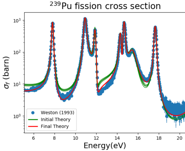
Fig. 11. ^{239}\text{Pu} resonance parameters adjustment on a fission cross section measurement. Theoretical/experimental comparisons before an after adjustment.
