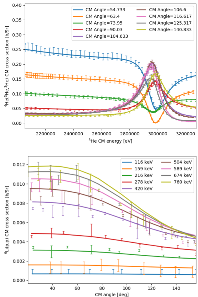
Fig. 13. Simultaneous analysis of measurements involving the same compound system. Up is the comparison of CONRAD on Barnard 1964 ^4\text{He}(^3\text{He},^3\text{He}) measurements. Bottom is the comparison of CONRAD (with the same model than previously) on Fasoli 1964 ^6\text{Li}(p,p) measurements.
