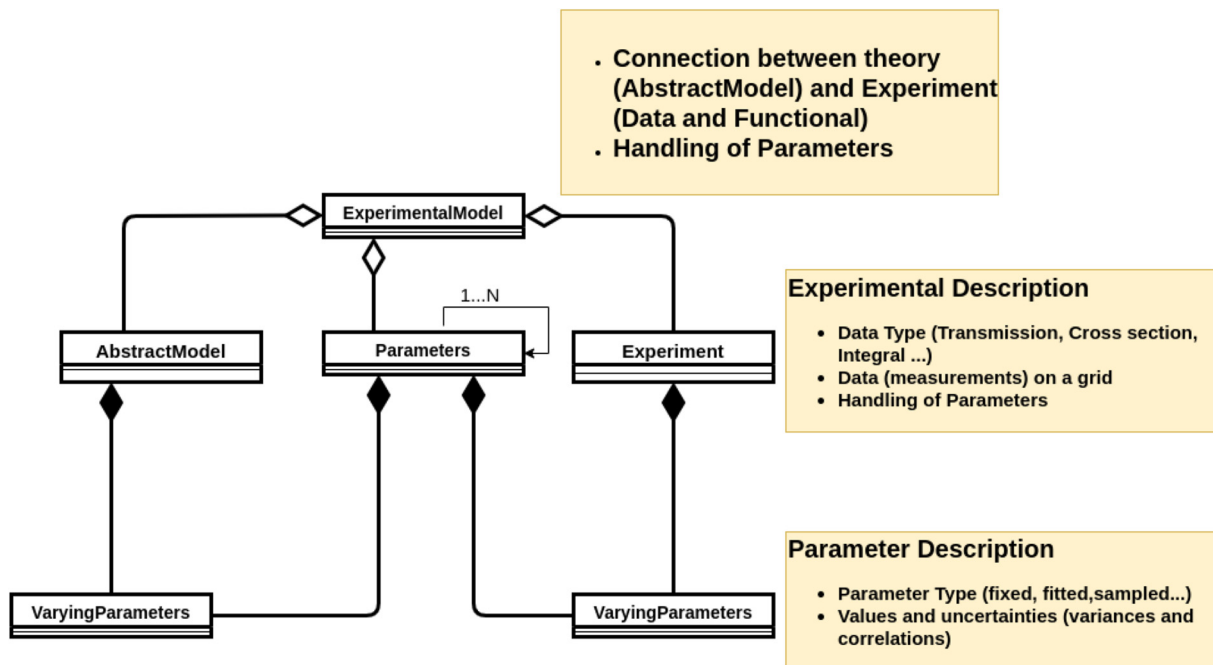
Fig. 2. Diagram description of CONRAD Experimentalmodel interface.
