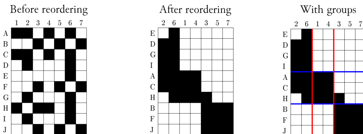
Figure 1: Using co-clustering to group students and items according to response patterns (adapted from Brault & Mariadassou, 2015, p.122)
