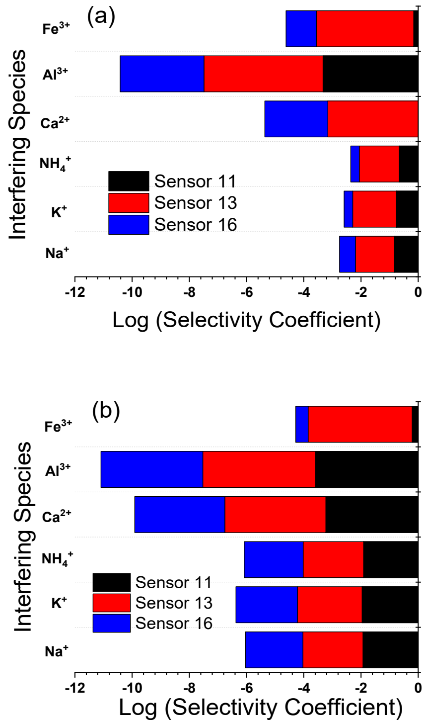
Figure 9. Log selectivity coefficient, \log K_{LF^{2+}, J^{z+}}^{\text{pot}} , determined by using SSM and MPM for a carbon paste electrode (CPE, sensor 11); PVC membrane coated on a carbon paste electrode (C-CPE, sensor 13); PVC/CD plasticized carbon paste electrode (P-CPE, sensor 16) at room temperature of 22 \pm 2 °C: (a) at pH 2.2; (b) at pH 4.1. The electrode compositions (% wt/wt ) are given in (Table 1).
