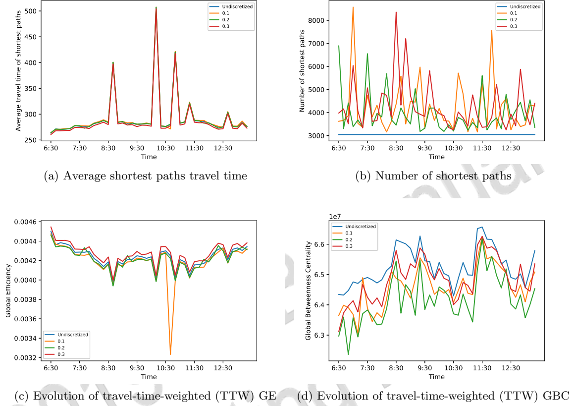
Figure 4: Evolution of the graph-based weighted metrics between 6:30am and 1:30pm for discretized weights [t, \alpha \cdot t] and different values of \alpha under normal conditions.
