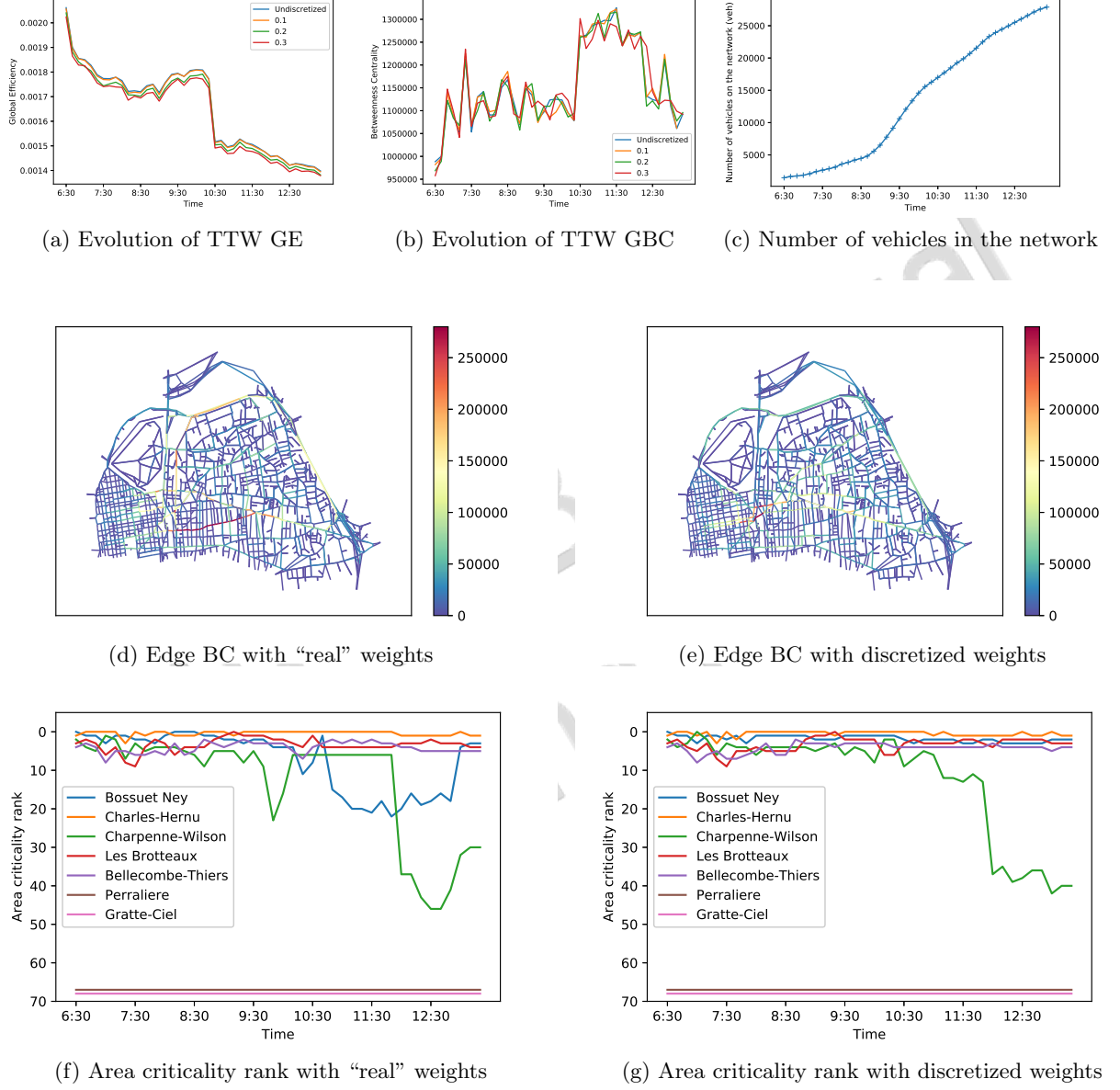
Figure 6: Evolution of the graph-based weighted metrics between 6:30am and 1:30pm for discretized weights [t, \alpha \cdot t] and different values of \alpha in presence of congestion at global and edges BC distributions at 8:30am and area rankig at local levels.
