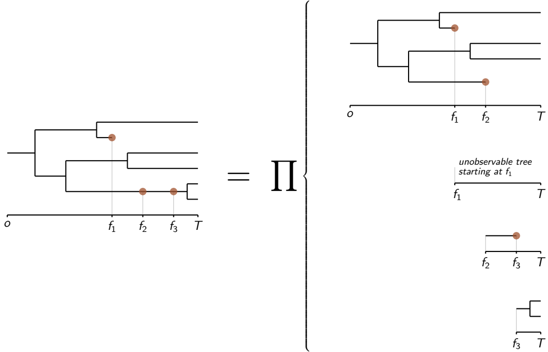
Figure 2: Decomposition of the probability density of a phylogenetic tree of extinct and extant taxa with fossils (figured by brown dots) as the product of the probability densities of “basic trees” by cutting it at each fossil find (adapted from Didier and Laurin, 2020).
