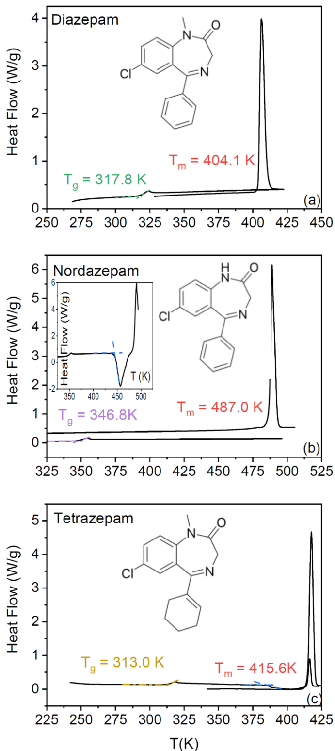
Figure 1. DSC traces of DIA (a), NOR (b), TETRA (c), obtained with a 10 \text{ K min}^{-1} heating/cooling rate. Upwards peaks are endothermic processes. Inset to (b): a different heating ramp acquired on amorphous NOR, where recrystallization is visible. The experimental determination of the glass transition, recrystallization, and melting temperatures are indicated with dashed lines.
