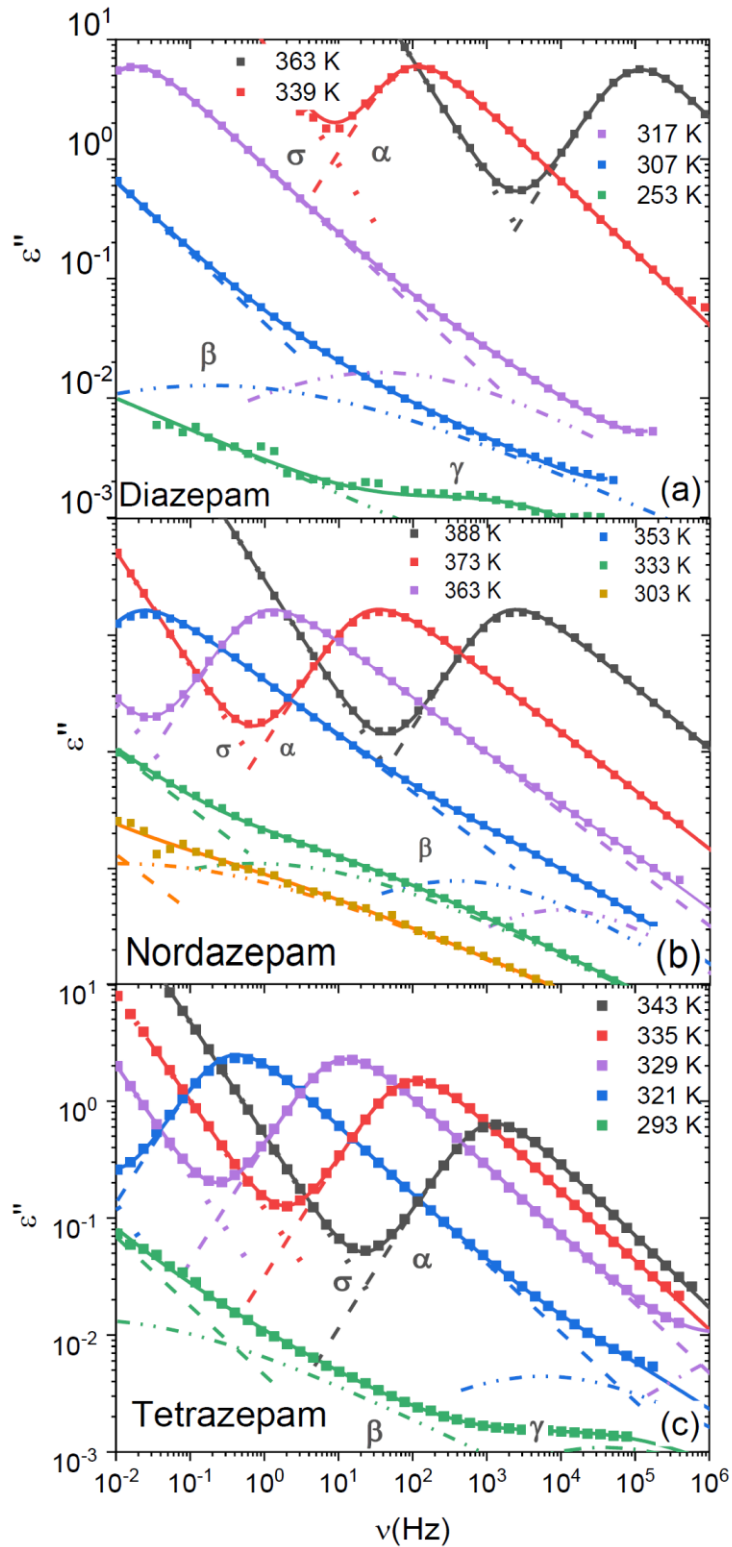
Figure 4. Loss spectra of amorphous DIA (a), NOR (b), TETRA (c) (markers), at selected temperatures as indicated in the legends, and their fits (continuous lines) as the sum of several Havriliak-Negami functions (dashed-dotted lines) and a DC conductivity background (dotted lines).
