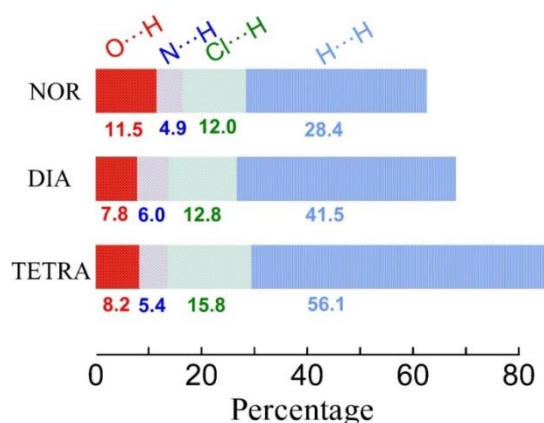
Figure 3. Contributions (in percentage) to the Hirshfeld surface areas of relevant intermolecular contacts: O...H, N...H and Cl...H as well as H...H to have a reference for TETRA, DIA and NOR compounds in the crystalline phase at room temperature as derived from the Hirshfeld surface area analysis (after ref 40).
