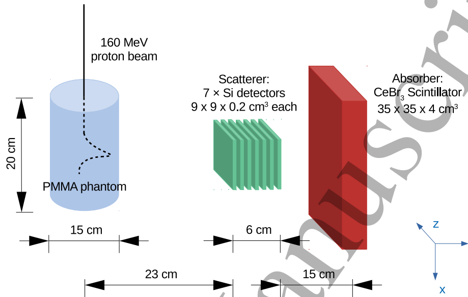
Figure 1: The geometry used in the GATE simulations. A Compton camera, comprised of 7 plane silicon detectors and a CeBr 3 scintillator, was positioned so as to detect prompt \gamma -rays generated in a polymethyl methacrylate (PMMA) phantom by an incident proton beam.
