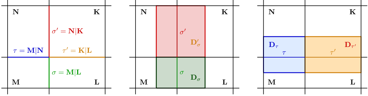
FIGURE 1. Primal and dual meshes and associated notations for the MAC case. - Left: the primal cells; the edges \sigma and \sigma' belong to \mathfrak{F}^{(1)} and the edges \tau and \tau' to \mathfrak{F}^{(2)} . - Center: the dual cells associated to \mathfrak{F}^{(1)} . - Right: the dual cells associated to \mathfrak{F}^{(2)} .
