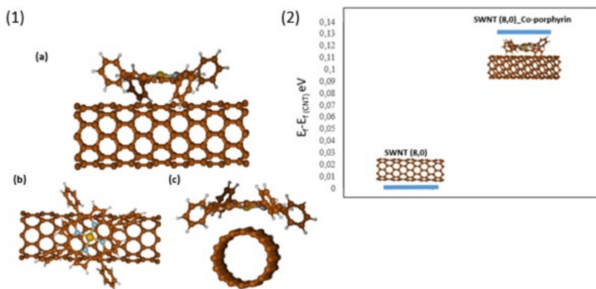
Figure 8. (1). Optimized geometry of the Co-Por adsorbed on the SWNT (8,0). (a) front view, (b) top view and (c) side view. (2). Fermi levels of SWNT (8,0) and SWNT (8,0)_Co-Por at the PBE0-D3/6-31G** level of theory using CRYSTAL.
