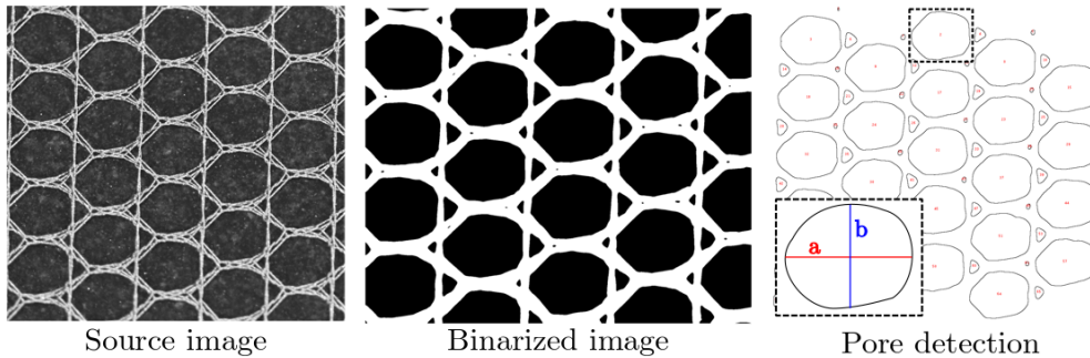
Figure 1: Pore size evaluation. The source image is binarized and pore contours detected.
