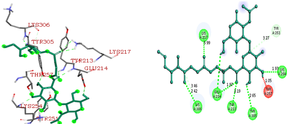
Fig.7. PLpro (PDB ID 6W9C)- 2DG Docking Complex 3D pose and 2D Interaction plot (-4.6Kcal/mol)
