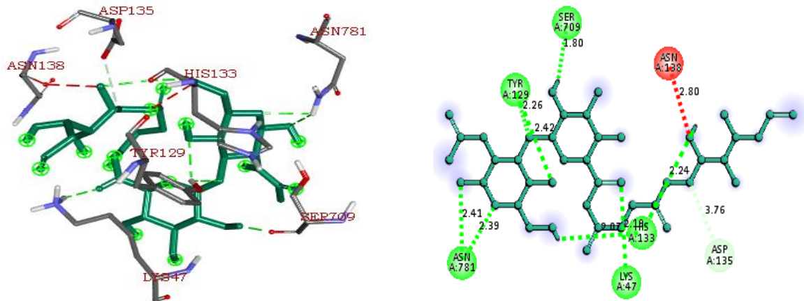
Fig.6. RdRp (PDB ID 6M71)- HA 2DG Docking Complex 3D pose and 2D Interaction plot (-7.2Kcal/mol)
