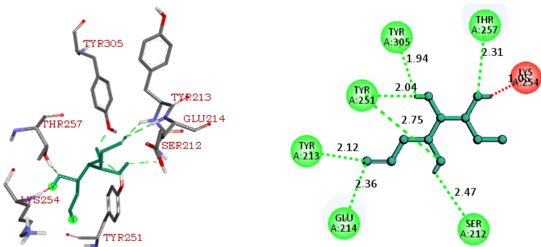
Fig.7. PLpro (PDB ID 6W9C)- 2DG Docking Complex 3D pose and 2D Interaction plot (-4.6Kcal/mol)
