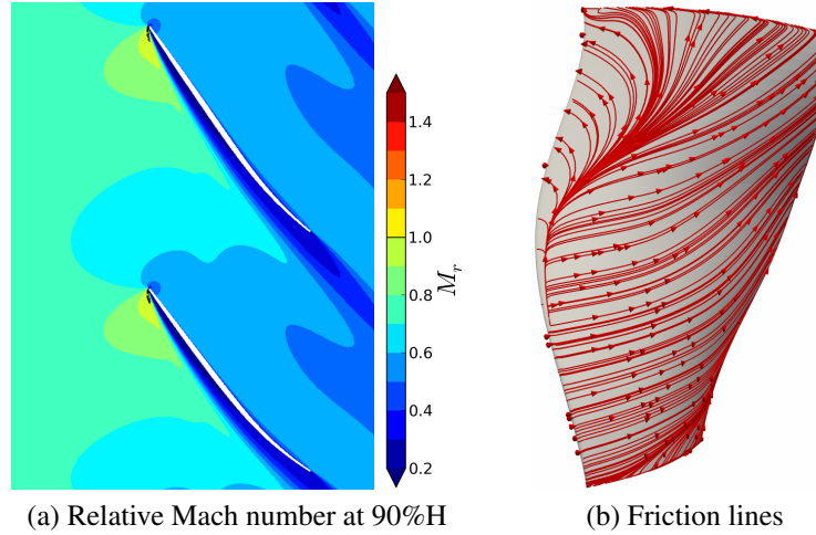
Figure 10: Steady flow at OP-D
