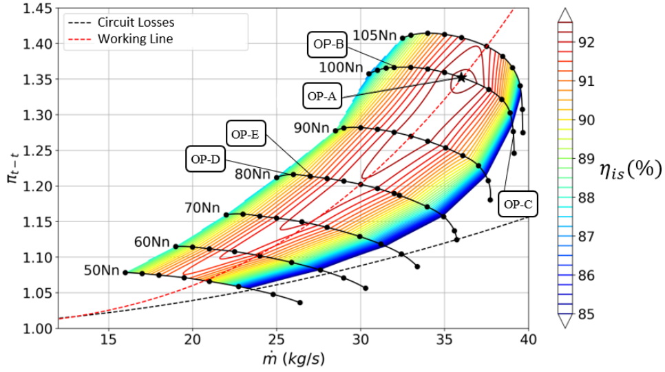
Figure 8: Compressor map with stability point of interest
