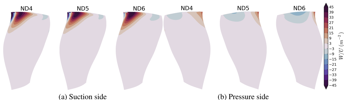
Figure 14: Local work OP-E, Mode 2ND(4-6)
