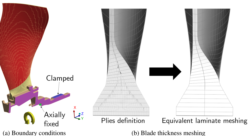
Figure 3: Mechanical model
