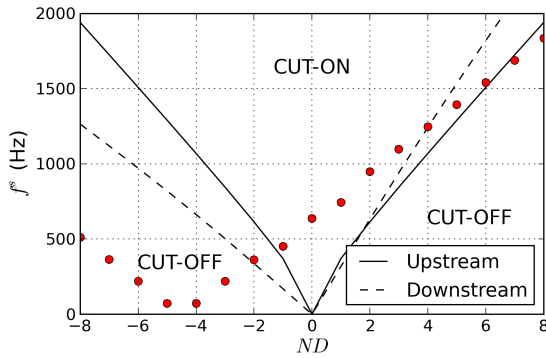
Figure 12: Mode 2 acoustic conditions at OP-D
