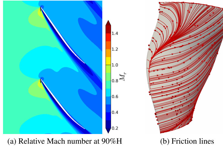
Figure 10: Steady flow at OP-D
