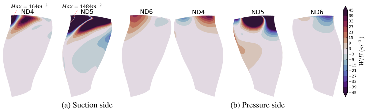
Figure 11: Local work at OP-D, Mode 2ND(4-6)
