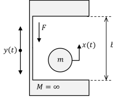
Figure 9: The dynamic model.
