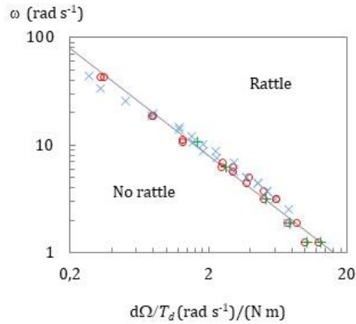
Figure 4: Theoretical rattle threshold master curve (black line) and rescaled experimental data. Drag torque T_d = 0.22 N m (+++++), T_d = 0.46 N m (ooooooo), T_d = 0.75 N m (xxxxxxx).
