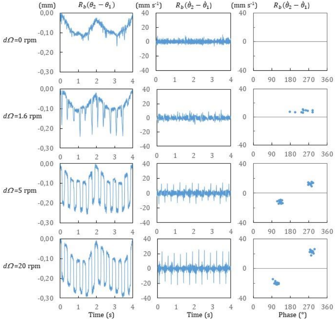
Figure 5: Impact response for increasing amplitude of velocity fluctuation \Delta\Omega . ( \Delta\Omega = 0, 1.6, 5 and 20 rpm). \Omega_0 = 30 rpm, \omega/2\pi = 3 Hz, T_d = 0.22 N m. Column 1: dynamic transmission error R_b(\theta_2 - \theta_1) , column 2: velocity dynamic transmission error R_b(\dot{\theta}_2 - \dot{\theta}_1) , column 3: Poincaré sections - impacting velocity vs. phase.
