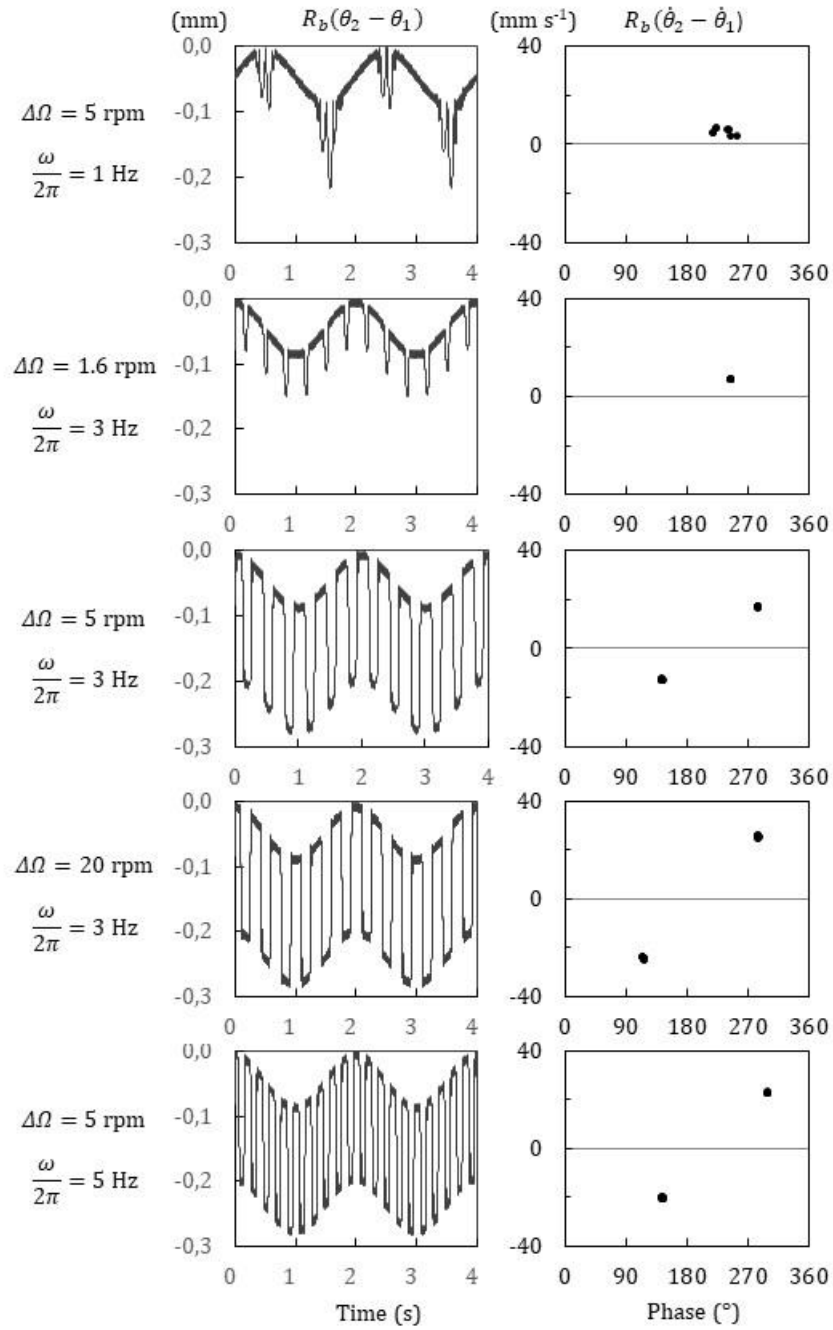
Figure 12: Relative dynamic response of the output gear in between the active and reverse flanks of the drive gear. Time history and Poincaré section. e = 0.5 , \Omega_0 = 30 \text{ rpm} , T_d = 0.22 \text{ N m} .
