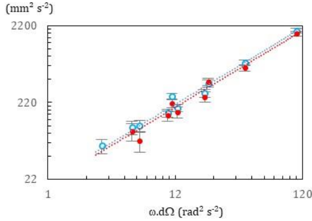
Figure 7: Mean value and standard deviation of the squared impacting velocity v_z^2 versus (\omega \cdot \Delta\Omega) .
