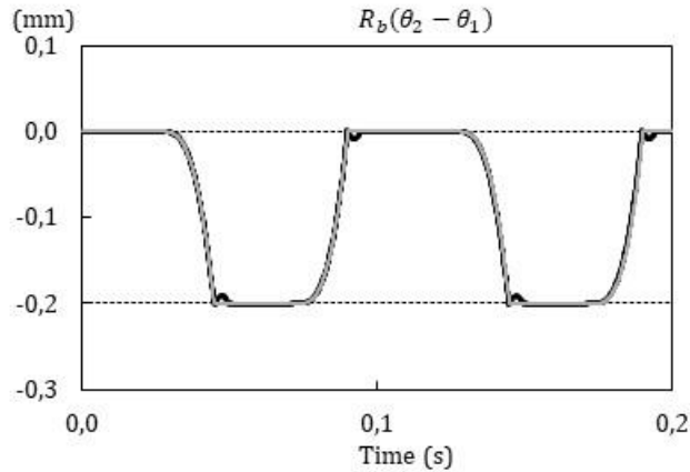
Figure 11: Relative dynamic response of the output gear in between the active and reverse flanks of the drive gear. Grey line: e = 0 . Black line: e = 0.3 . b = 200 \mu\text{m} , T_d = 0.22 \text{ N m} , \Delta\Omega = 4 \text{ rpm} and
