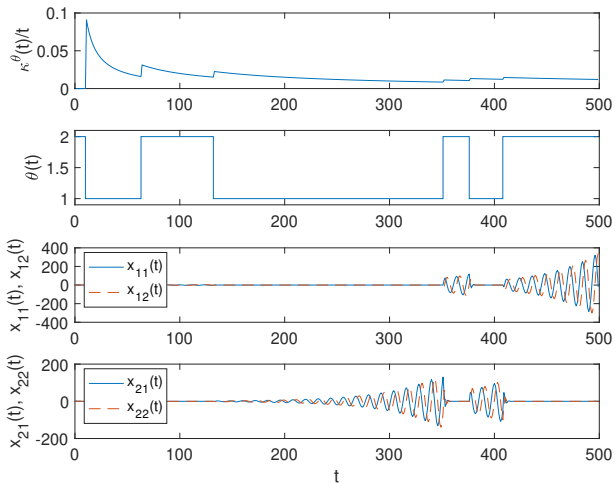
Fig. 7. Time evolution of the synchronization error x(t) and the switching signal \theta(t) for a shuffling rate lower than \gamma^* = 0.06 .
