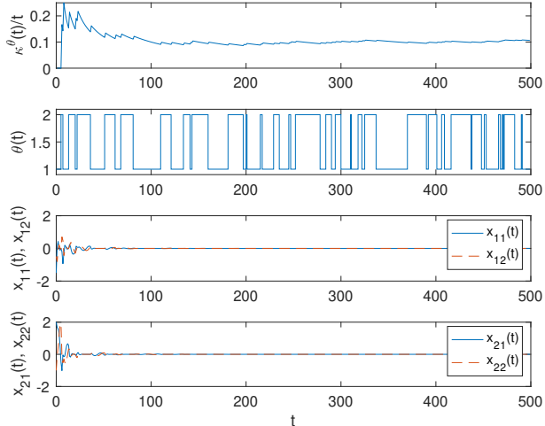
Fig. 6. Time evolution of the synchronization error x(t) and the switching signal \theta(t) for a shuffling rate higher than \gamma^* = 0.06 .
