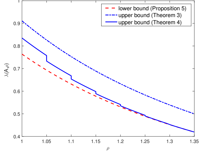
Fig. 4. Lower and upper bounds on the \rho -SJSR for (29).
