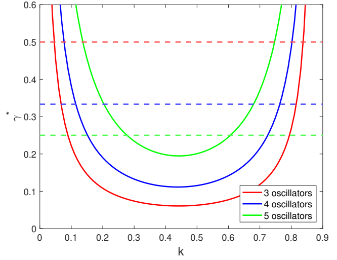
Fig. 5. Minimal shuffling rate \gamma^* as a function of the control gain k and of the number of oscillators m + 1 .
