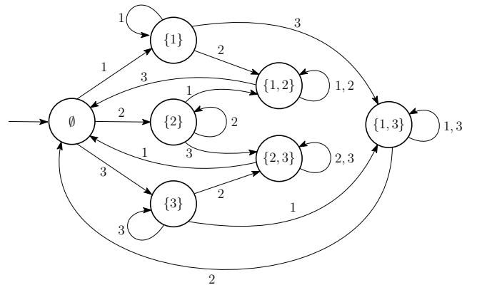
Fig. 3. Automaton describing the dynamics of \eta in (28) for m = 3 . State labels correspond to the value of \eta , transition labels correspond to the value of \theta .
