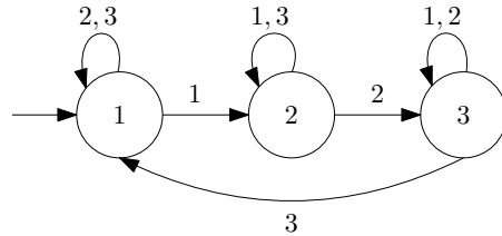
Fig. 2. Automaton describing the dynamics of \eta in (24) for m = 3 . State labels correspond to the value of \eta , transition labels correspond to the value of \theta .
