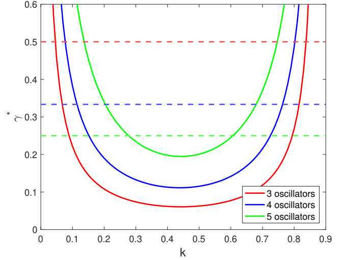
Fig. 5. Minimal shuffling rate \gamma^* as a function of the control gain k and of the number of oscillators m + 1 .
