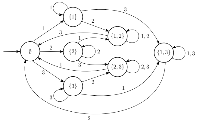
Fig. 3. Automaton describing the dynamics of \eta in (28) for m = 3 . State labels correspond to the value of \eta , transition labels correspond to the value of \theta .
