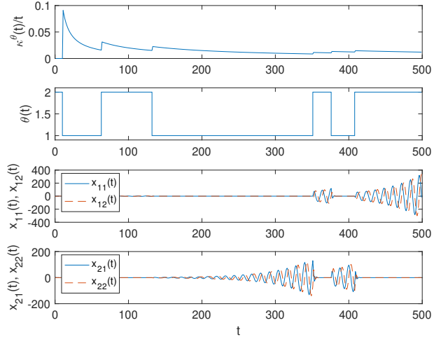
Fig. 7. Time evolution of the synchronization error x(t) and the switching signal \theta(t) for a shuffling rate lower than \gamma^* = 0.06 .
