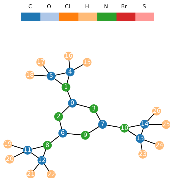
Figure 7: Triethylenemelamine.
