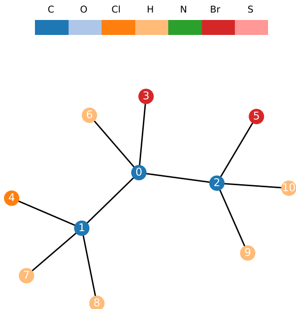
Figure 3: 1,2-Dibromo-3-Chloropropane.
