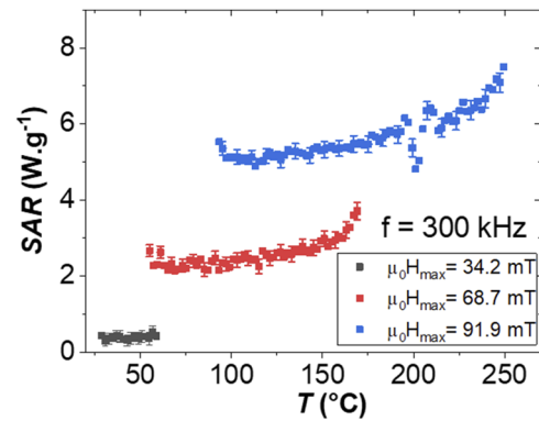
FIG. 7. Heating power as a function of the temperature for a sample of NEG for three different magnetic fields at a frequency f = 300 kHz. Since we deduce the first 4 s of measurement, which brings the material to a higher temperature if a higher field is applied, the starting temperature of the treated data is higher with a higher applied field.
