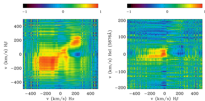
Fig. 11. Correlation matrices between different lines. The color range corresponds to the value of the linear correlation coefficient between the different velocity bins of the line profiles. Perfect anticorrelation corresponds to -1 (black), no correlation to 0 (light blue), and a perfect correlation to 1 (orange).
