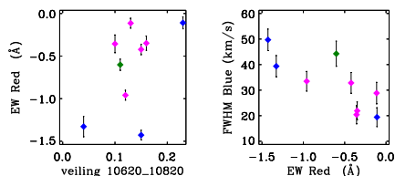
Fig. 17. Parameters of the He I 10830 Å line. Left: Equivalent width of redshifted absorption as a function of the veiling measured close to the line. Right: FWHM of the blueshifted absorption. Colors represent different rotational cycles: dark green - cycle 5; purple - cycle 6; blue - cycle 7.
