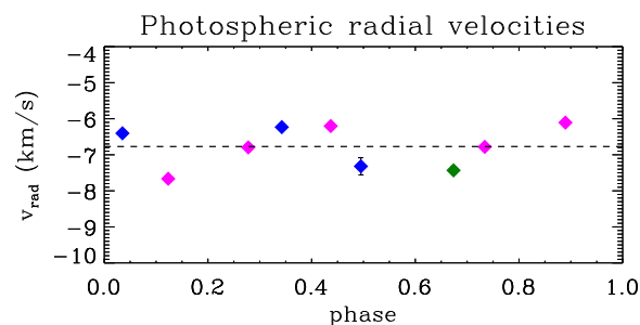
Fig. 12. Radial velocity of photospheric lines obtained with SPIRou data and in phase with the same ephemeris from Alencar et al. (2012) and Donati et al. (2007). The radial velocity is the mean of all the radial velocities measured on the same night, and the error bar is its respective standard deviation. The colors represent different cycles: dark green - cycle 5; purple - cycle 6; and blue - cycle 7. The dashed line is the mean value of all observed nights.
