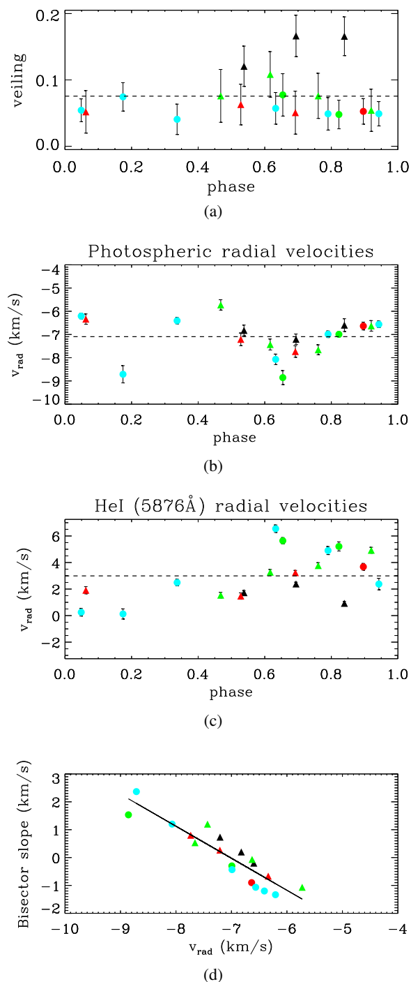
Fig. 4. Veiling (a) and the radial velocity (b) of photospheric lines in phase with the ephemeris from Alencar et al. (2012) and Donati et al. (2007). The veiling and radial velocity correspond to mean values obtained from all spectroscopic regions used in the calculations. The error bars come from the standard deviations. (c) He I 5876Å line radial velocities. (d) Bisector slope as a function of the radial velocities. The colors represent different cycles: black - cycle 0; green - cycle 1; red - cycle 2; and light blue - cycle 3. The dashed line is the mean value of all observations. Triangles are ESPaDOnS data, and circles are HARPS data.
