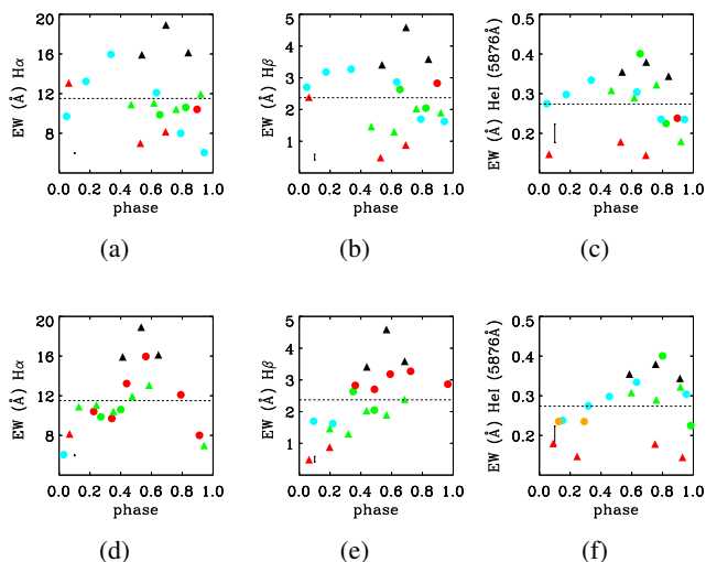
Fig. 10. Equivalent widths of emission lines as a function of the rotational phase. Top: Phases computed with the stellar rotational period (6.53 days). Bottom: Periods of 8.5, 8.0, and 6.0 days used to reconstruct the cycles for, respectively, H \alpha , H \beta , and He I 5876Å. Colors represent different rotational cycles. We note that the phase and the duration of a cycle are different in the top and bottom plots. The error bar on the plots are the mean of the 3\sigma equivalent width uncertainties (see text).
