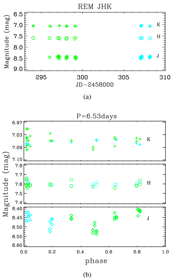
Fig. 2. Photometric JHK light curves obtained with the REM telescope as a function of observing date (a) and phase (b). We calibrated the magnitudes using the 2MASS JHK magnitudes of a reference star (see text). The statistical uncertainties on the magnitudes are smaller than the symbols.
