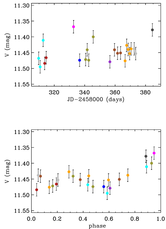
Fig. 3. V-band light curve of V2129 Oph from ASAS-SN photometry. Top: Direct light curve. Bottom: Light curve folded in phase with the ephemeris given in Eq. (1). The colors represent different rotation cycles.
