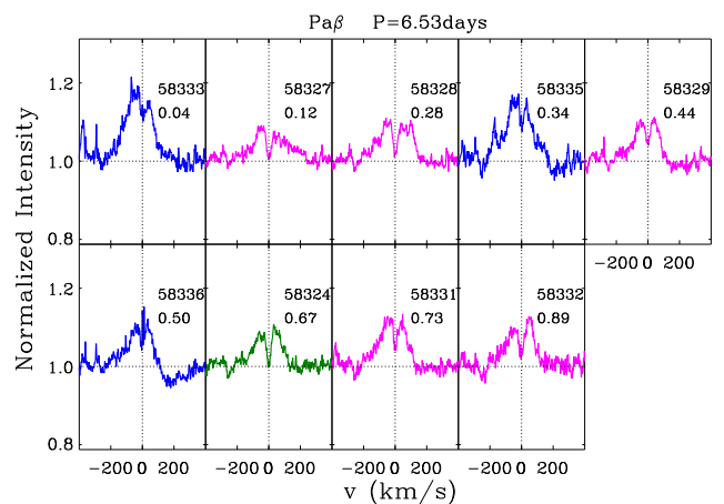
Fig. 15. Pa \beta emission line profiles obtained with the SPIRou spectrograph, organized by phase. The phase and the JD of the observations are written in each panel. The colors represent different rotational cycles.
