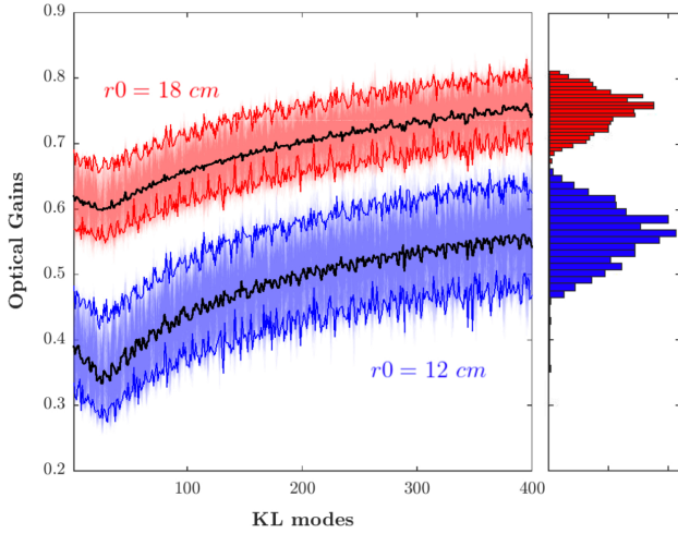
Fig. 2. Variability of closed-loop OG. For given system parameters we compute T_\phi for 1000 phase realisations in two seeing configurations: r0 = 18 cm and r0 = 12 cm. The variability of the frame-by-frame OG is shown in the histogram in the right panel and by the highlighted extreme OG curves for each r0 case.
