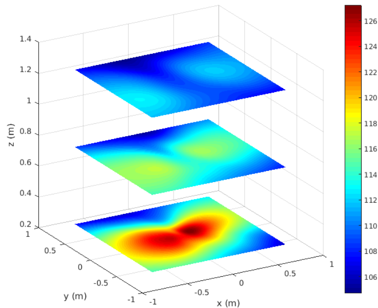
Figure 3. Acoustic patterns in dB for the steady state vibration regime (for t > 1 s) on different horizontal planes at 0.25 m, 0.75 m and 1.25 m.
