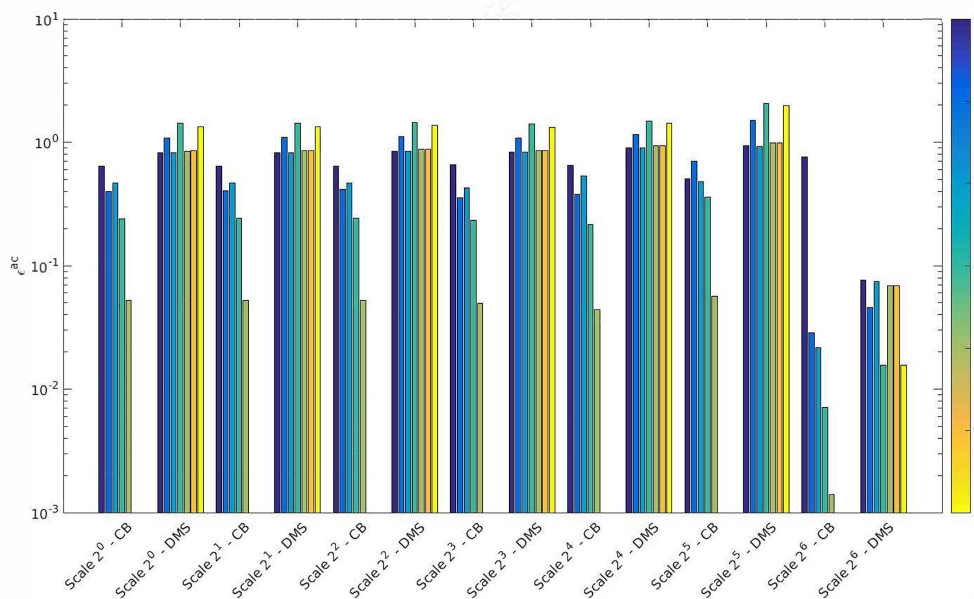
Figure 7. Values of \epsilon^{ac} for \mu = 0.8 —horizontal planes (definition of the color bar for "Scale 2^j —CB": 1 \rightarrow \gamma = 0.5 , 2 \rightarrow \gamma = 1 , 3 \rightarrow \gamma = 1.25 , 4 \rightarrow \gamma = 1.5 , 5 \rightarrow \gamma = 2.5 ; definition of the color bar for "Scale 2^j —DMS": 1 \rightarrow N_{DMS} = 50 , 2 \rightarrow N_{DMS} = 100 , 3 \rightarrow N_{DMS} = 150 , 4 \rightarrow N_{DMS} = 220 , 5 \rightarrow N_{DMS} = 500 , 6 \rightarrow N_{DMS} = 750 , 7 \rightarrow N_{DMS} = 1000 ).
