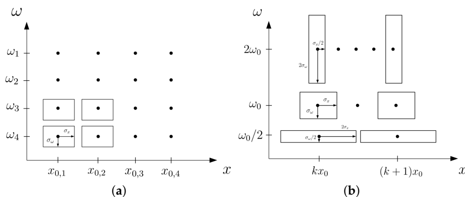
Figure 5. Diagram of observation cells and variable mesh in the 2D dimension x/\omega (a) Fourier representation (b) Wavelet representation.
