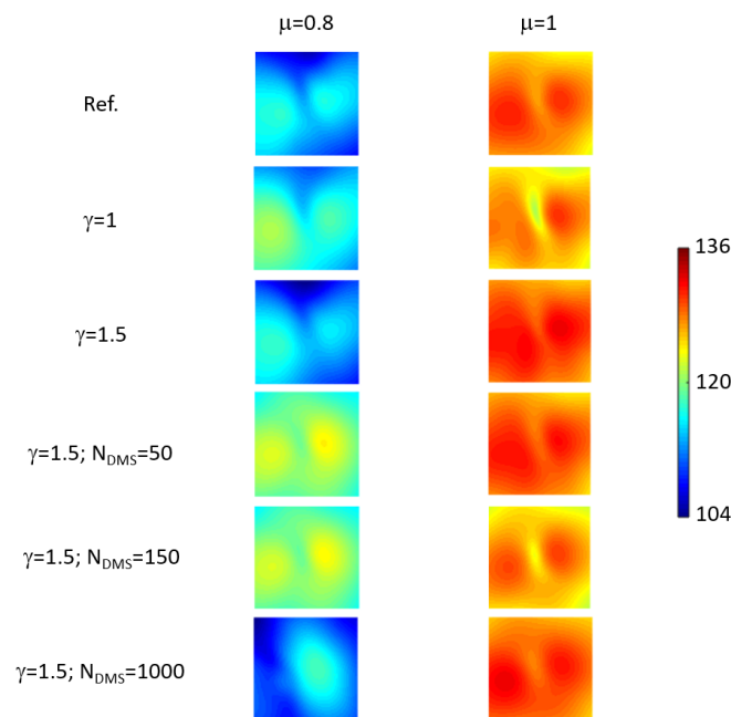
Figure 10. Acoustic patterns on the horizontal plane at the distance of 0.75 m in the direction Z for different C&B and DMS reductions, scale in dB.
