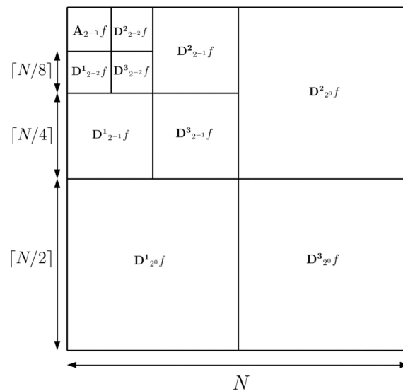
Figure 6. Illustration of the 2D wavelet decomposition of a pattern of size N for three iterations, according to Mallat’s algorithm.
