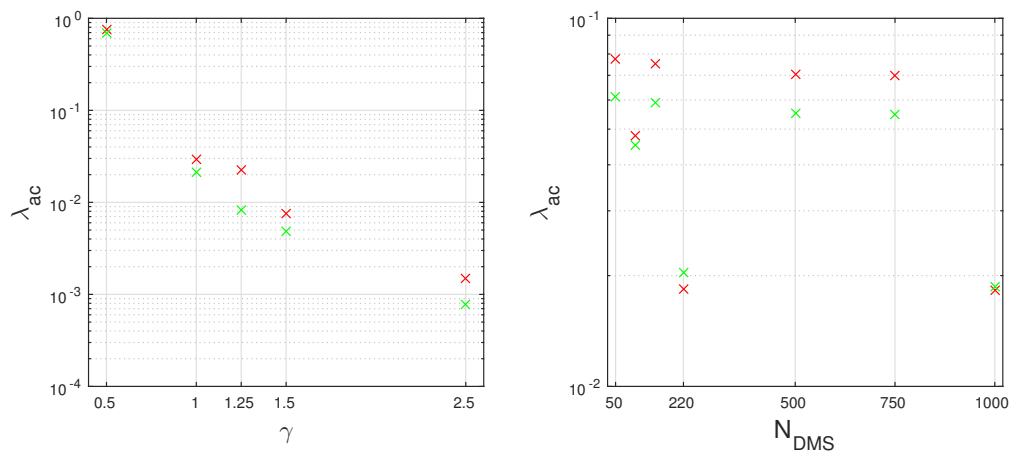
Figure 9. Values of \lambda_{ac} at \mu = 0.8 for horizontal planes (red) and vertical planes (green).
