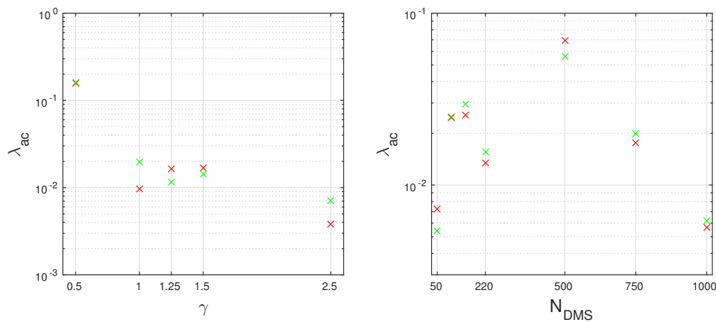
Figure 11. Values of \lambda_{ac} at \mu = 1 for horizontal planes (red) and vertical planes (green).
