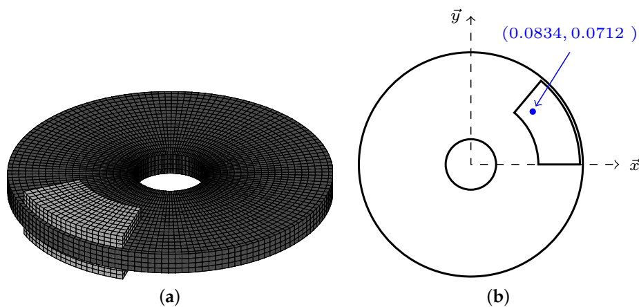
Figure 1. Simplified brake system under study (a) Finite Element Model (b) Position of the selected point for the description of the nonlinear dynamic response.
