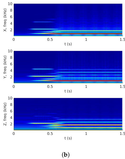
Figure 2. Transient nonlinear behavior of the system for \mu = 0.8 (a) time responses and (b) spectrograms.
