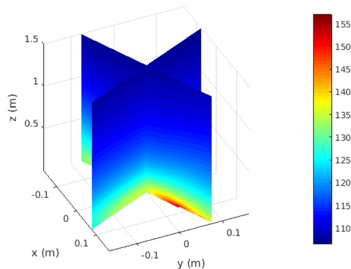
Figure 4. Acoustic patterns in dB for the steady state vibration regime (for t > 1 s) on two vertical planes.
