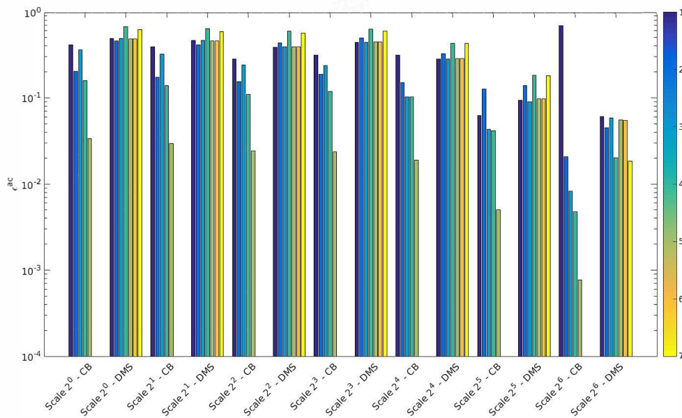
Figure 8. Values of \epsilon^{ac} for \mu = 0.8 —vertical planes. Definition of the color bar for “Scale 2^j —CB”: 1 \rightarrow \gamma = 0.5, 2 \rightarrow \gamma = 1, 3 \rightarrow \gamma = 1.25, 4 \rightarrow \gamma = 1.5, 5 \rightarrow \gamma_{colora} = 2.5 ; definition of color bar for “Scale 2^j —DMS”: 1 \rightarrow N_{DMS} = 50, 2 \rightarrow N_{DMS} = 100, 3 \rightarrow N_{DMS} = 150, 4 \rightarrow N_{DMS} = 220, 5 \rightarrow N_{DMS} = 500, 6 \rightarrow N_{DMS} = 750, 7 \rightarrow N_{DMS} = 1000 .
