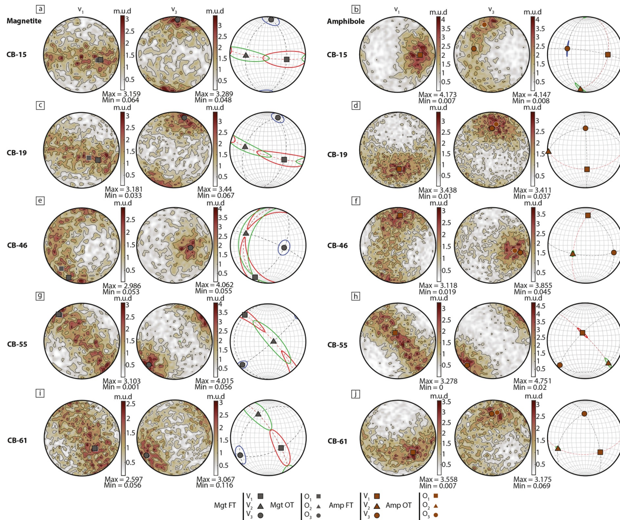
Figure 5. Lower-hemisphere equal-area Schmidt nets showing v_1 and v_3 orientations and the fabric and orientation tensors for magnetite and amphibole populations for sample CB-15C2, CB-19A1, CB-46A1, CB-55A1 and CB-61B2. The v_1 and v_3 axes are represented with multiples of uniform distribution (M.U.D.) contour plots. The mean fabric tensors with confidence ellipses of the tensor analyses created with Tomofab are plotted in lower-hemisphere equal-area Schmidt nets. Confidence ellipses (95%) were calculated with Jelinek statistics.
