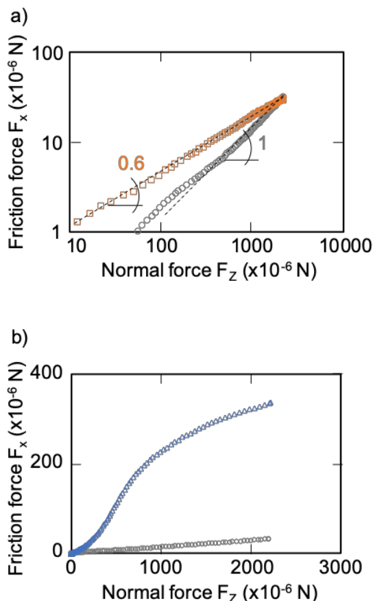
Figure 3. Influence of the molecular architecture on the friction force variation for fatty acids (a) for the straight alkyl chain, stearic acid ( \circ ) and elaidic acid ( \square ) in logarithmic scale, and (b) for the bent alkyl chain oleic acid ( \triangle ) in linear scale. The stearic acid data were also reported in (b) for sake of comparison.
