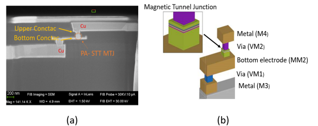
Fig. 2. Scanning electron microscope (SEM) image of a SPINTEC PA-SST MTJ (a). The corresponding PA-SST MTJ model created in the TRADCARE simulation environment (b).
