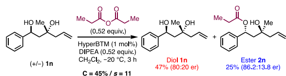
Scheme 5. KR of 1,3-Diol 1n
