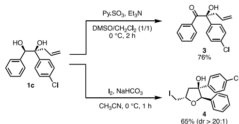
Scheme 6. Postfunctionalizations of Diol 1c
