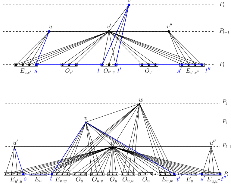
Figure 7: The proof of Theorem 3.10: in blue is the path S = usPtv't'' , when v' is of type 1 (top) and when v' is of type 2 (bottom)
