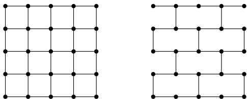
Figure 1: A grid and a wall
