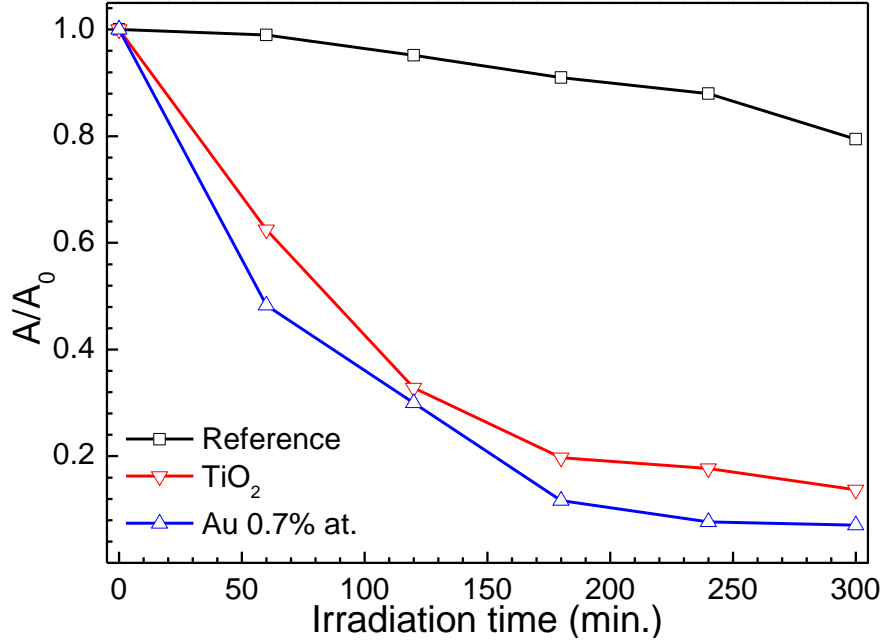
Figure 6. A/A_0 as a function of time for pure \text{TiO}_2 and Au- \text{TiO}_2 films with 0.7% at. Au deposited at 8 Pa. The error bars are included within the point size.
