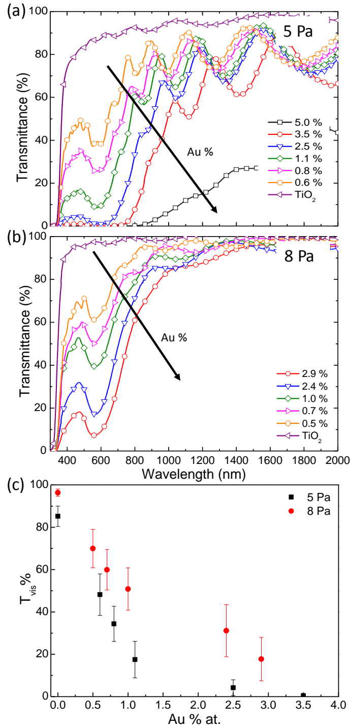
Figure 5. Optical transmittance of annealed Au-TiO 2 films deposited at (a) 5 Pa and (b) 8 Pa with different Au contents. (c) Average transmittance of annealed samples in the visible range (390-750nm) as a function of Au content at both deposition pressures.
