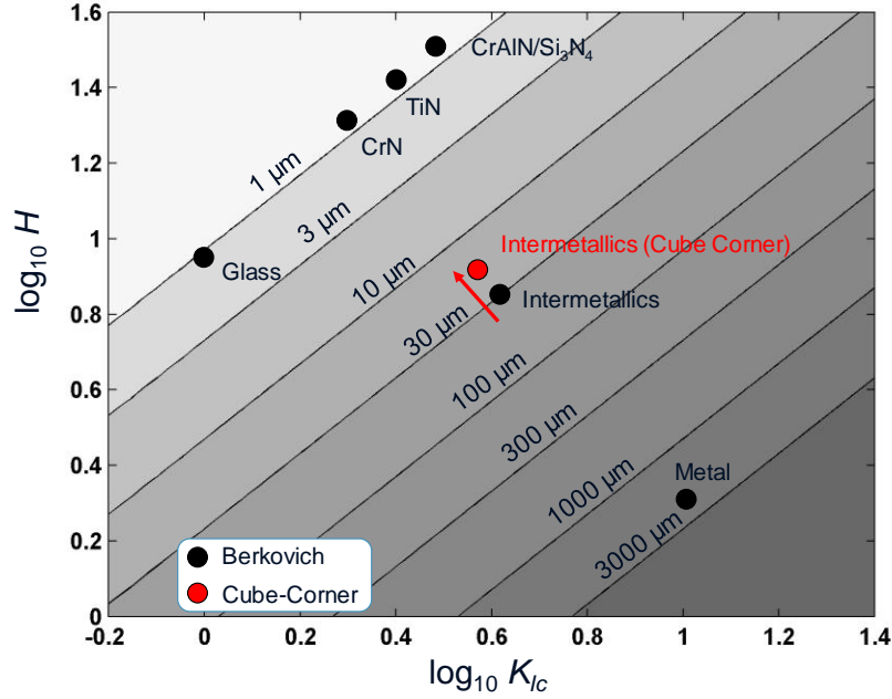
Fig. 6: A practical selection map showing that this method could be reliably applied to ceramics and some intermetallics [32].
