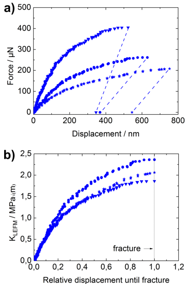
Fig. 19: (a) Force-displacement curves for soft-oriented cantilevers. The unloading slopes were estimated to be the same as the individual loading slopes. Slight changes in the geometrical dimensions like moment arm or beam width cause different force levels and displacements until the point of brittle fracture. Therefore, the respective stress intensity factors as a function of the “Relative displacement until fracture” are shown in (b).
