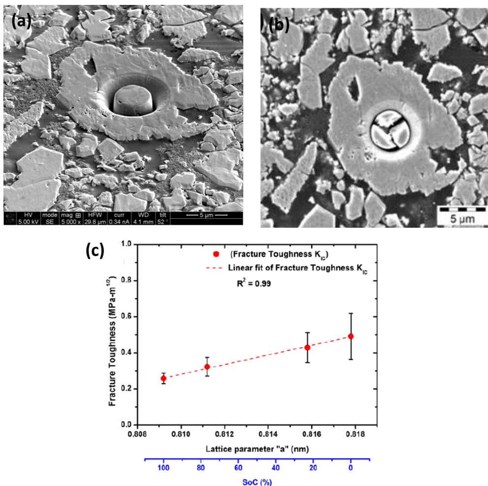
Fig. 8: (a,b) FIB-milled micro-pillars before and after splitting of Li x Mn 2 O 4 crystals embedded in polymeric matrix; (c) fracture toughness as a function of lattice parameter [39].
