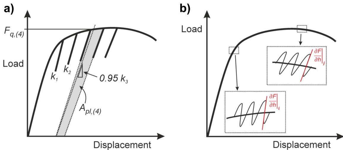
Fig. 17: Schematic load-displacement curves to describe the J -Integral testing procedure: (a) method with partial unloading segments to determine the contact stiffness k_i and the relevant quantities A_{pl,(i)} and F_{q,(i)} and (b) continuous stiffness technique which allows continuous recording of the contact stiffness.
