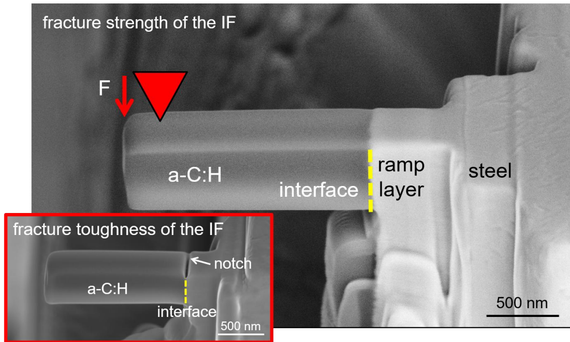
Fig. 13: (a) SEM images of micro-cantilevers prepared for fracture strength and toughness testing of the interface between a-C:H and the Cr bond coating [77].
