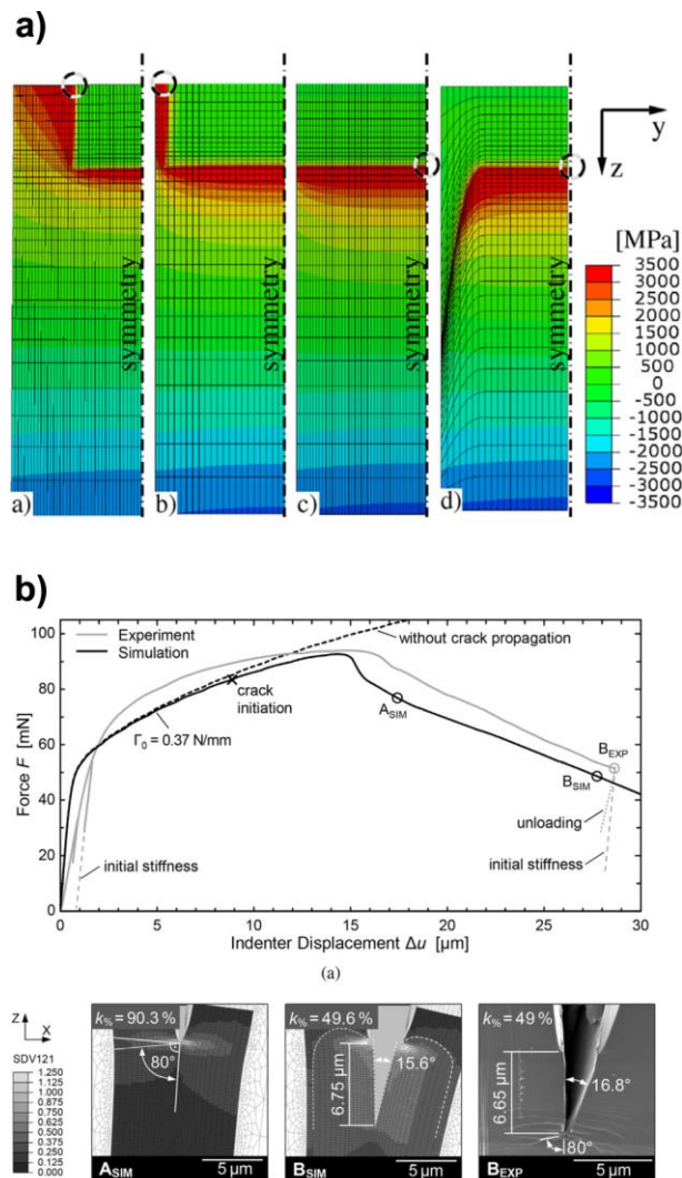
Fig. 11: FE simulations as tool to guide crack design and link simulations with experiments. (a) Effect of material bridges, straight through notch and “over-fibbing” on the ( \sigma_{11} ) stress distribution ahead of a crack in a rectangular cantilever, after [52] and (b) comparison of simulated and experimental fracture data of chevron-notched tungsten single crystal cantilevers showing plastic deformation and stable crack propagation, after [48].
