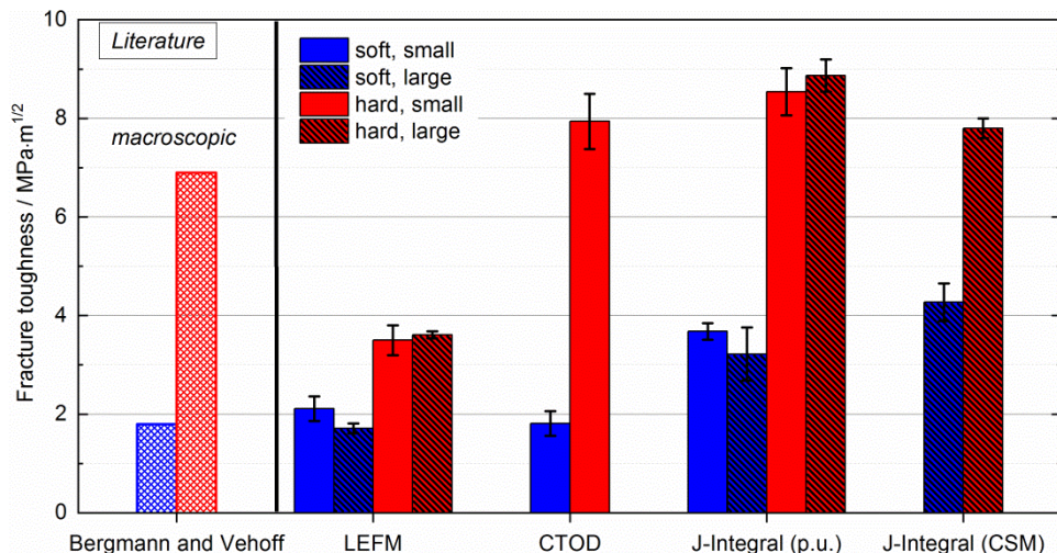
Fig. 22: Overview of fracture toughness data as evaluated by means of the different techniques; “p.u.” means partial unloading; literature data taken from [104] and “small” and “large” characterize the different cantilever sizes, which were investigated in the studies presented here.
