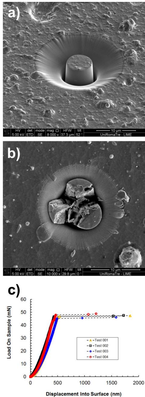
Fig. 2: (a) Example of a CrAlN/Si 3 N 4 pillar before splitting. (b) Example of a CrN pillar after splitting. (c) Load-displacement curves for CrN pillars, highlighting the critical load ( P_c ) corresponding to the crack 'popping out' to the side surface, and pillar splitting [31].
