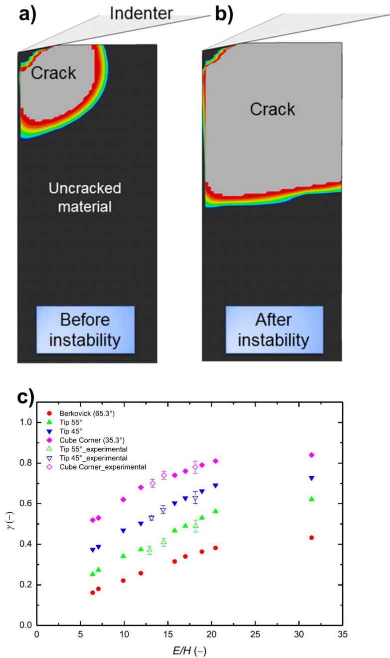
Fig. 3: (a,b) Crack geometries in a representative pillar splitting test just before and just after the instability load, respectively [32]. (c) \gamma (gamma) coefficient as a function of E/H for different tip geometries. The solid and empty symbols represent, respectively, FEM simulations and experimental data [35].
