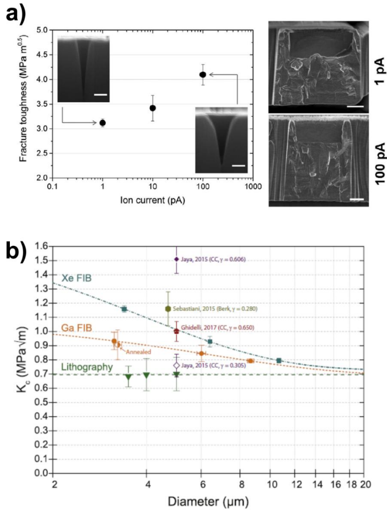
Fig. 23: a) Fracture toughness of CrN micro-cantilevers as a function of gallium ion current during notching. SEM images of FIB-polished cross sections of notches milled at 1 pA and 100 pA (inset, scale bar 100 nm), and HR-SEM images of the fractured cantilever surface post-fracture for 1 and 100 pA ion currents (scale bar 500 nm), after [34]. b) Variation of K_c as a function of pillar size for different production methods with indenter geometry (CC – cube corner, Berk – Berkovich) and \gamma coefficient [36].
