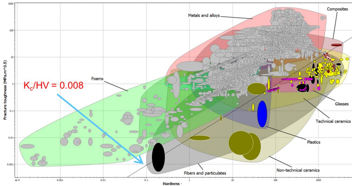
Fig. 7: Ashby selection chart identifying those materials with K_c/HV < 0.008 , which is the estimated minimum threshold for having unstable crack propagation during a pillar splitting experiment.
