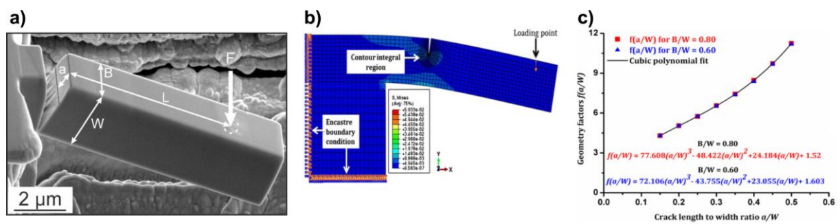
Fig. 10: (a) SEM image of a fractured cantilever in a NiAl single crystal, (b) FE model for the determination of the geometry function, shown in (c) for different a/W aspect ratios [57].
