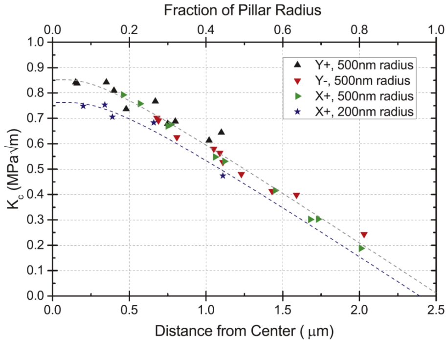
Fig. 5: Apparent fracture toughness as a function of distance to the center of the pillar with the offset orientation direction and the indenter tip radius noted [36].
