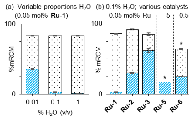
Figure 1. Impact of water on mRCM. (a) For Ru-1 at 0.5 h. (b) For various catalysts at 2 h (except Ru-6 : 24 h). * Ru-5 , Ru-6 : 60 °C, 0.01 atm. 33 For tabulated data, see Table S1.
