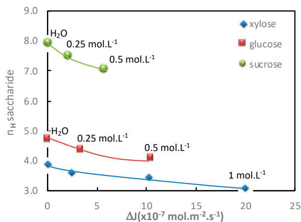
Figure 4. Impact of the electrolyte concentration. Correlation between the saccharide hydration number, n H , and the saccharide additional flux, Δ J , in the presence of Na 2 SO 4 . Saccharide = 1 mol·L -1 ; diffusion mode; T = 25 °C.
