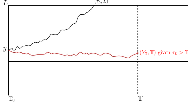
Figure 2: Two typical trajectories of continuous diffusion.
