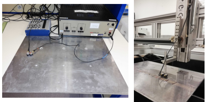
Figure 4: Pictures showing the experimental setups for Scenario 1 (left) and Scenario 3 (right).
